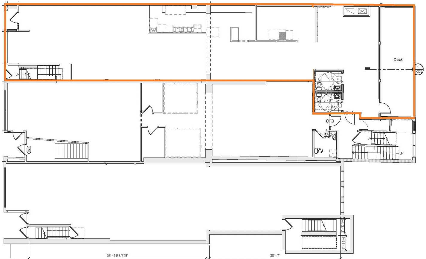
1 Level 1 Floor Plan A-110 4" 8" 12" 3/16" = 1'-0"
