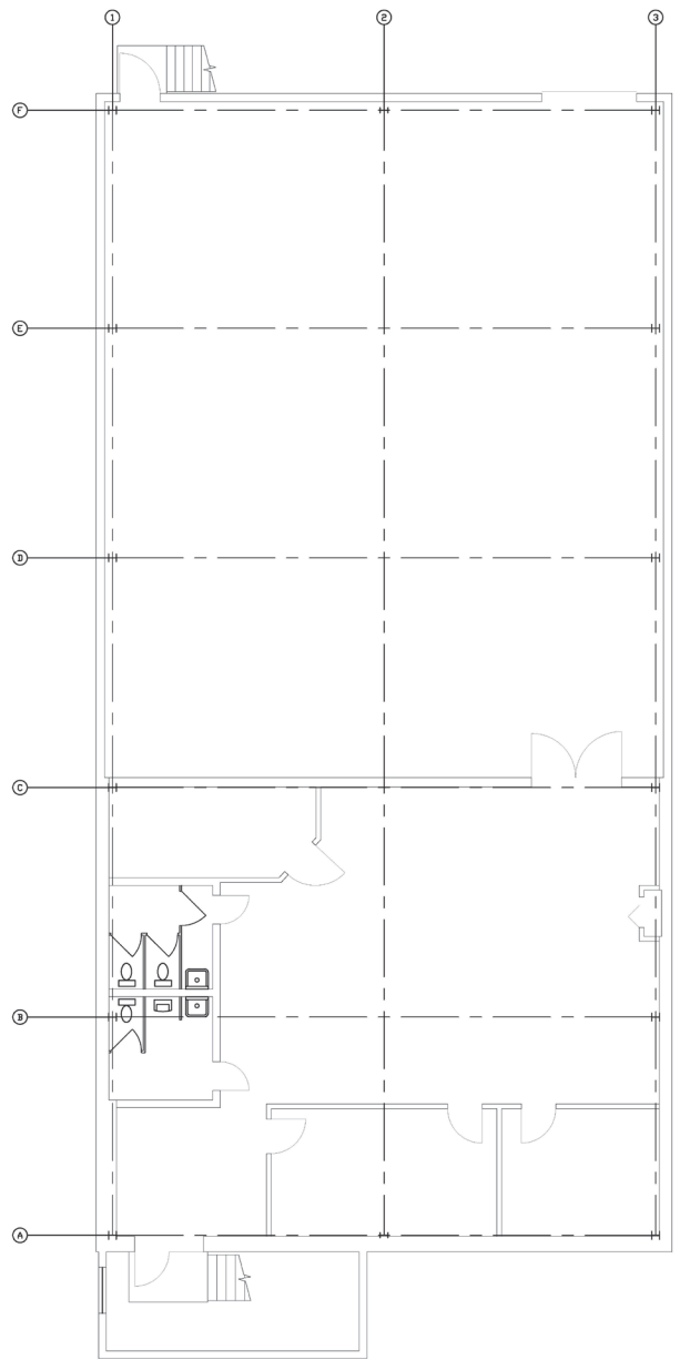
Ⓐ ARCHITECTURAL PLAN - 2ND FLOOR
