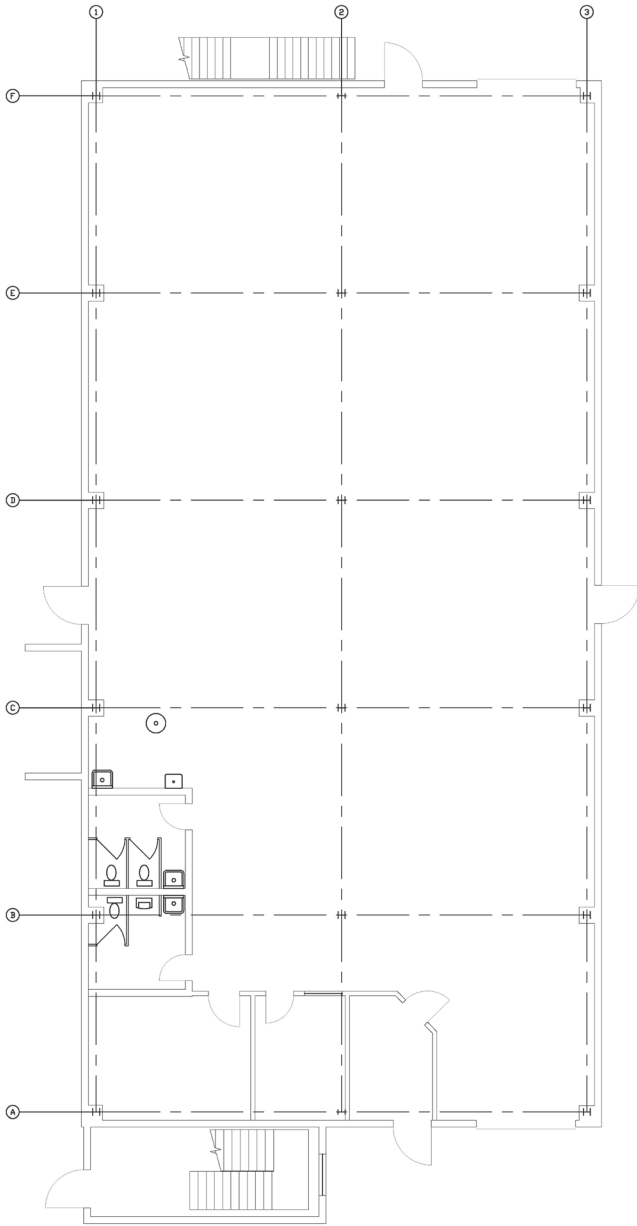
Ⓐ ARCHITECTURAL PLAN - 1ST FLOOR
