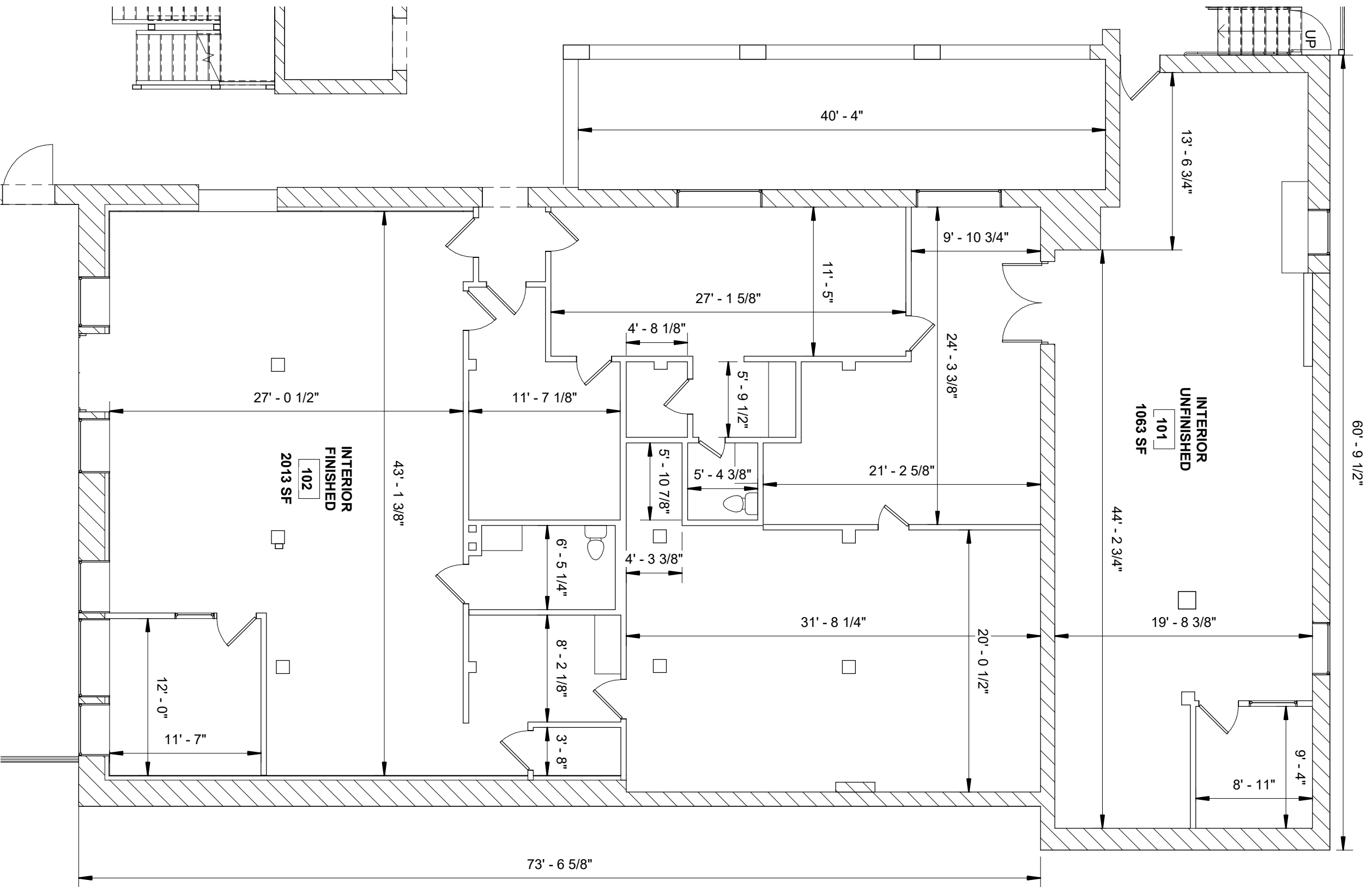
1 LEASEABLE COMMERCIAL SPACE 003 1/8" = 1'-0"
