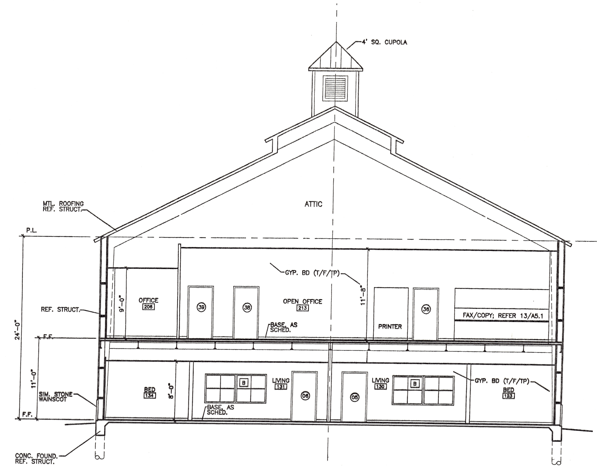
03 BUILDING SECTION
