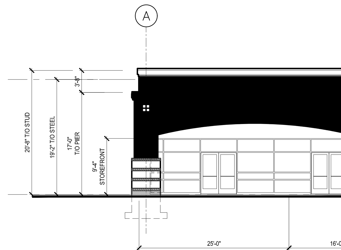
PARTIAL FRONT ELEVATION SCALE \frac{1}{8}"=1'-0"
