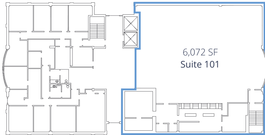
1st Floor
