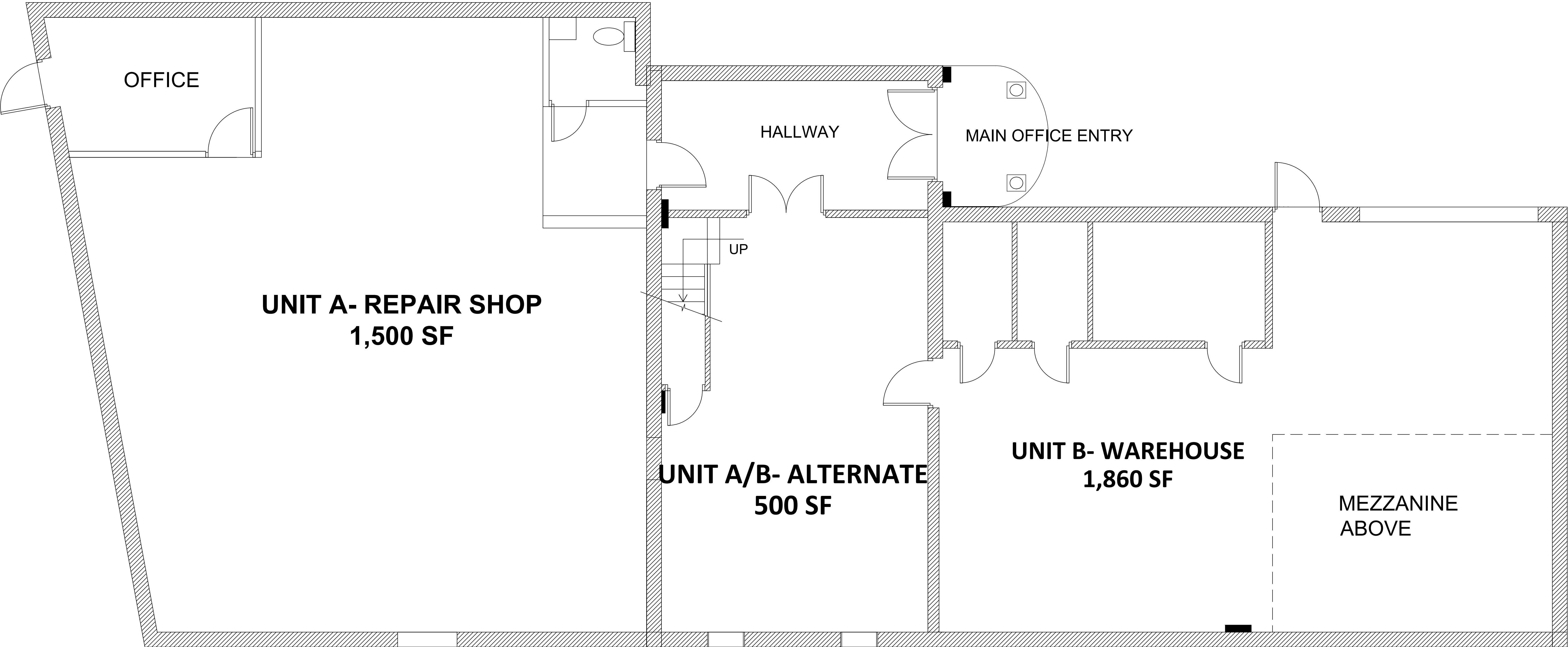
First Floor Plan W S → N
