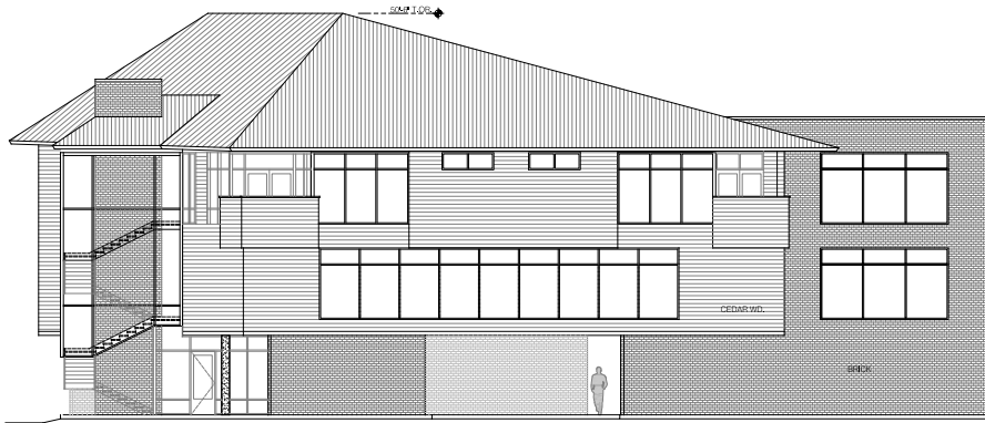
① NORTH ELEVATION 1/8" = 1'-0"
