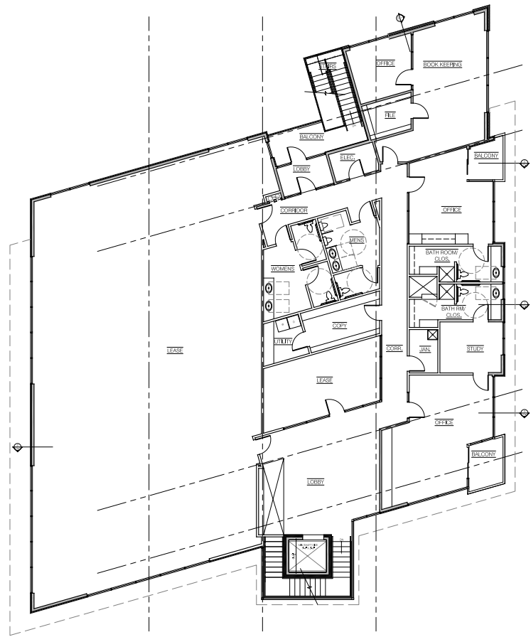
NORTH ② THIRD FLOOR PLAN 1/8" = 1'-0"
