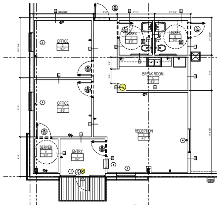
OFFICE FLOOR PLAN | BUILDINGS 4, 8 AND 9
