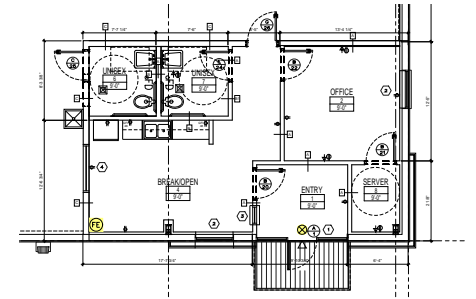
OFFICE FLOOR PLAN | BUILDINGS 6 AND 7
