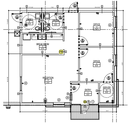
OFFICE FLOOR PLAN | BUILDINGS 2, 3 AND 10
