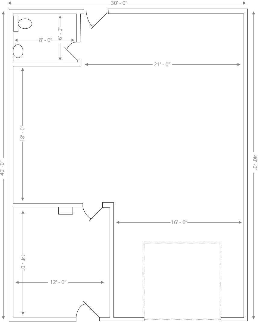
Typical Suite
