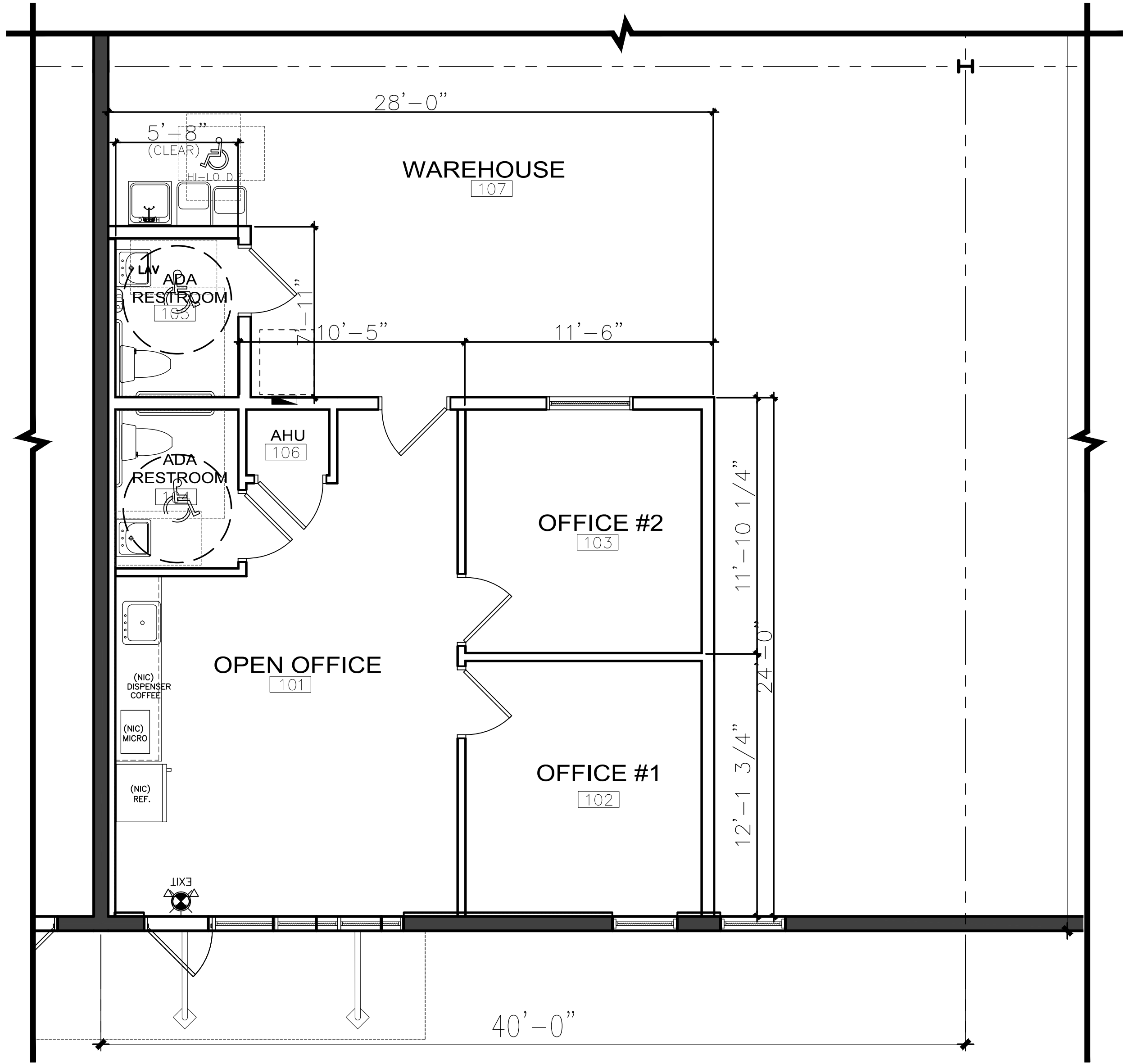
BUILDING 18 TYPICAL TENANT OFFICE PLAN SCALE: 1/4"=1'-0"
