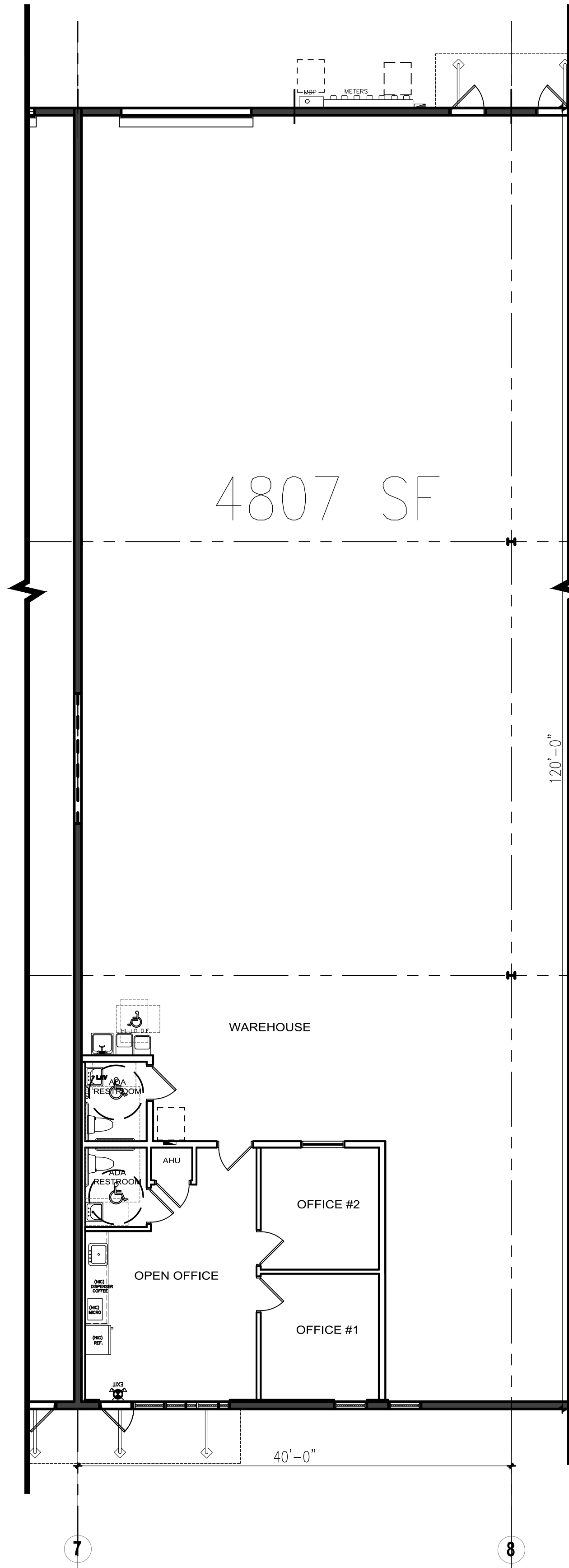
BUILDING 18 TYPICAL TENANT FULL BAY DEPTH PLAN SCALE: 1/8"=1'-0"
