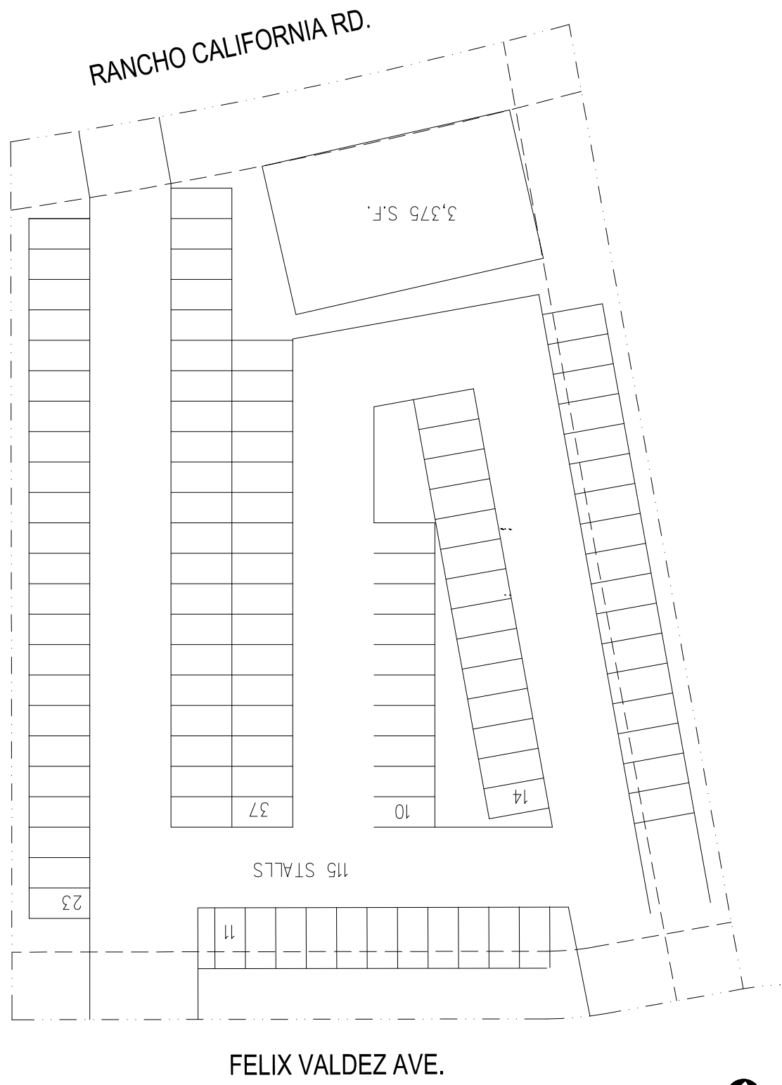
SCHEME B - 1ST FLOOR PLAN
