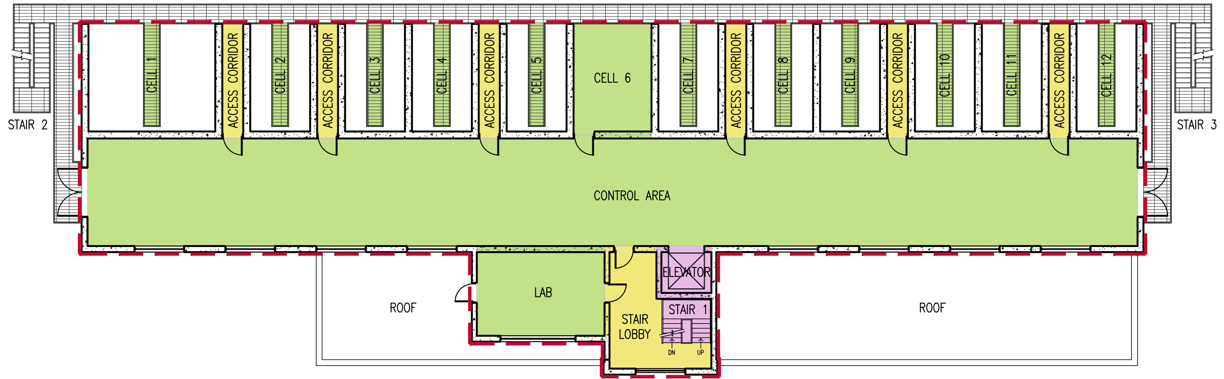
1 SECOND FLOOR PLAN SCALE: 1/16" = 1'-0"
