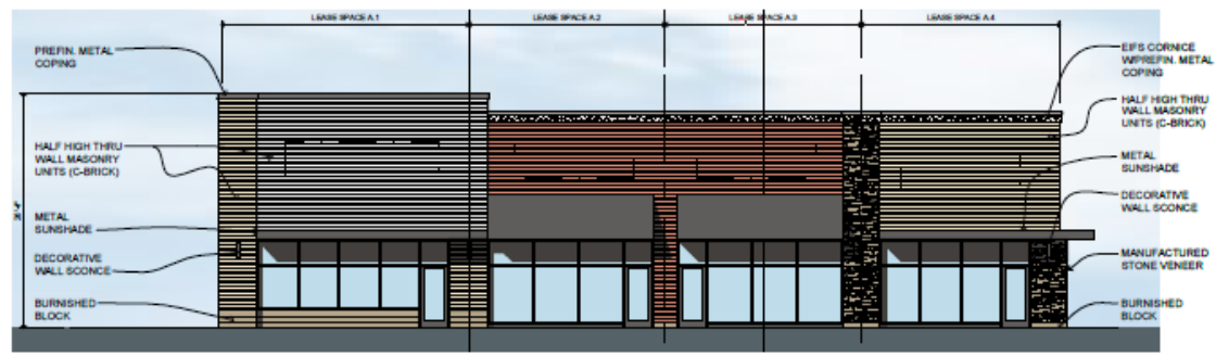
Bldg. A - South Elevation 1/8" = 1'-0"
