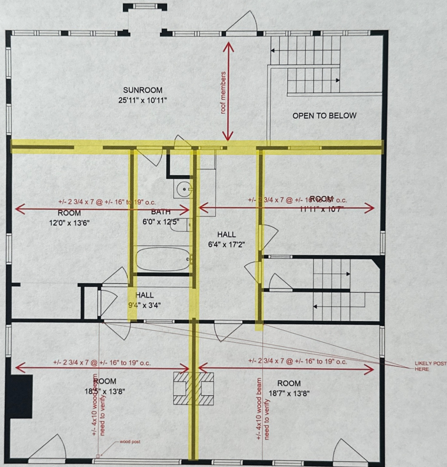
SECOND FLOOR FRAMING FRAMING
