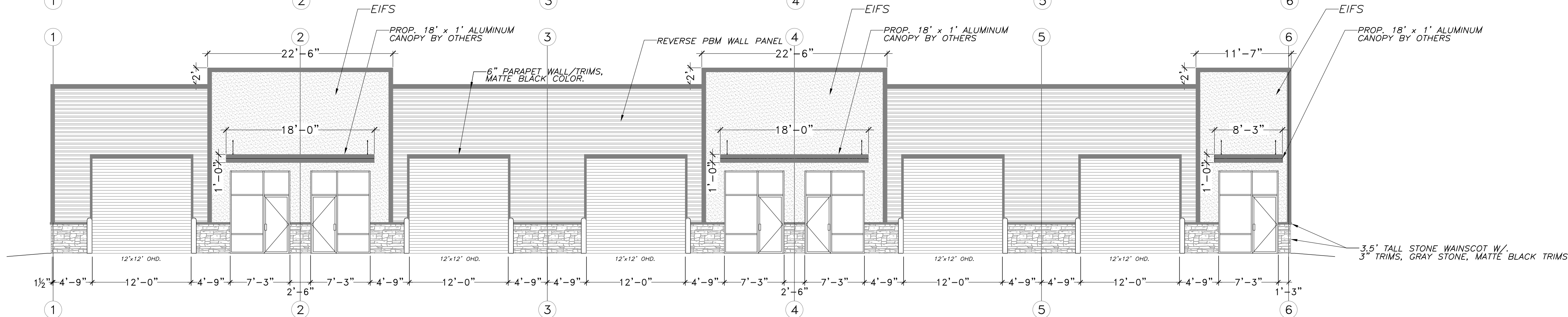
METAL OFFICE WAREHOUSE EAST ELEVATION 1/8"=1'-0"
