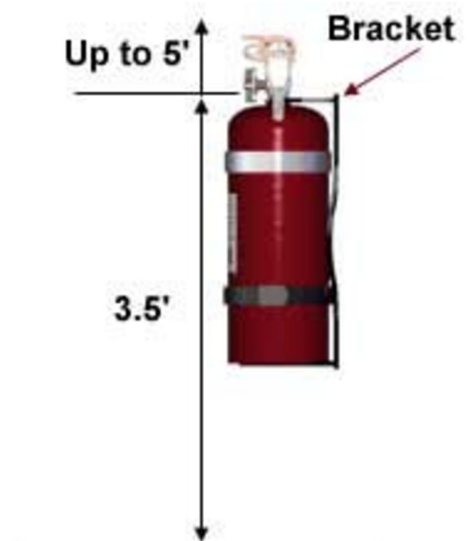
PORTABLE 2-A FIRE EXTINGUISHER PLACEMENT NTS
