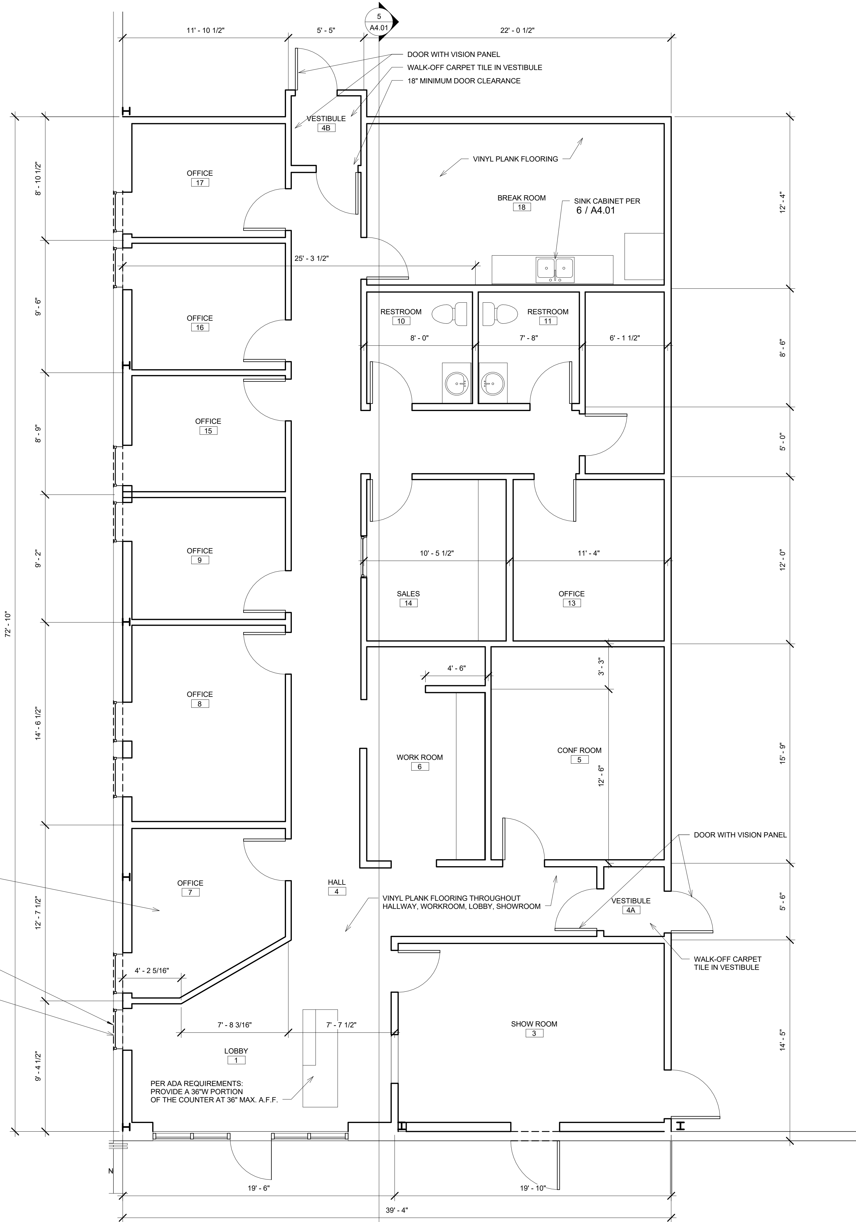
1 ENLARGED OFFICE PLAN 1/4" = 1'-0"
