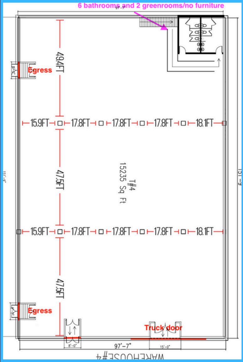
STAGE 4 - 15,235 SF
