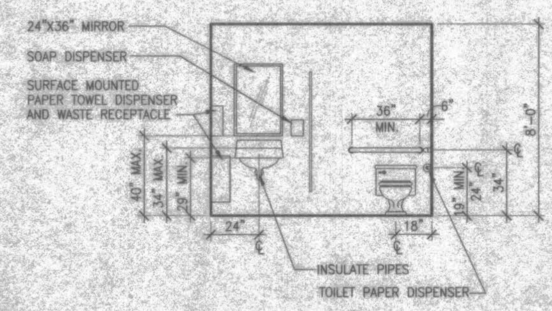
ELEVATION SCALE 1/4" = 1'-0" 2 A101
