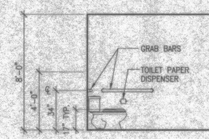
ELEVATION SCALE 1/4" = 1'-0" 3 A101
