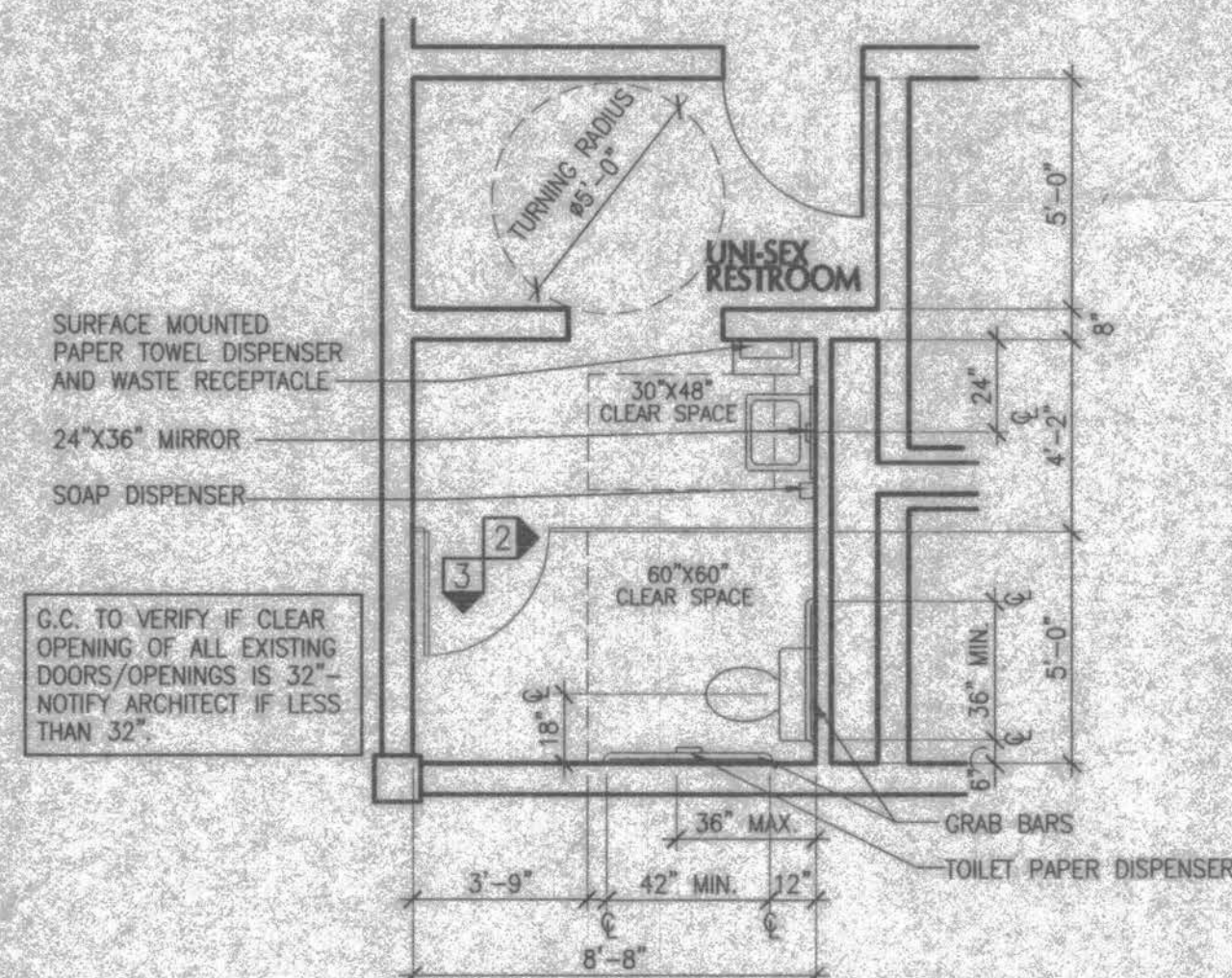
ENLARGED PLAN SCALE 1/4" = 1'-0" 1 A101
