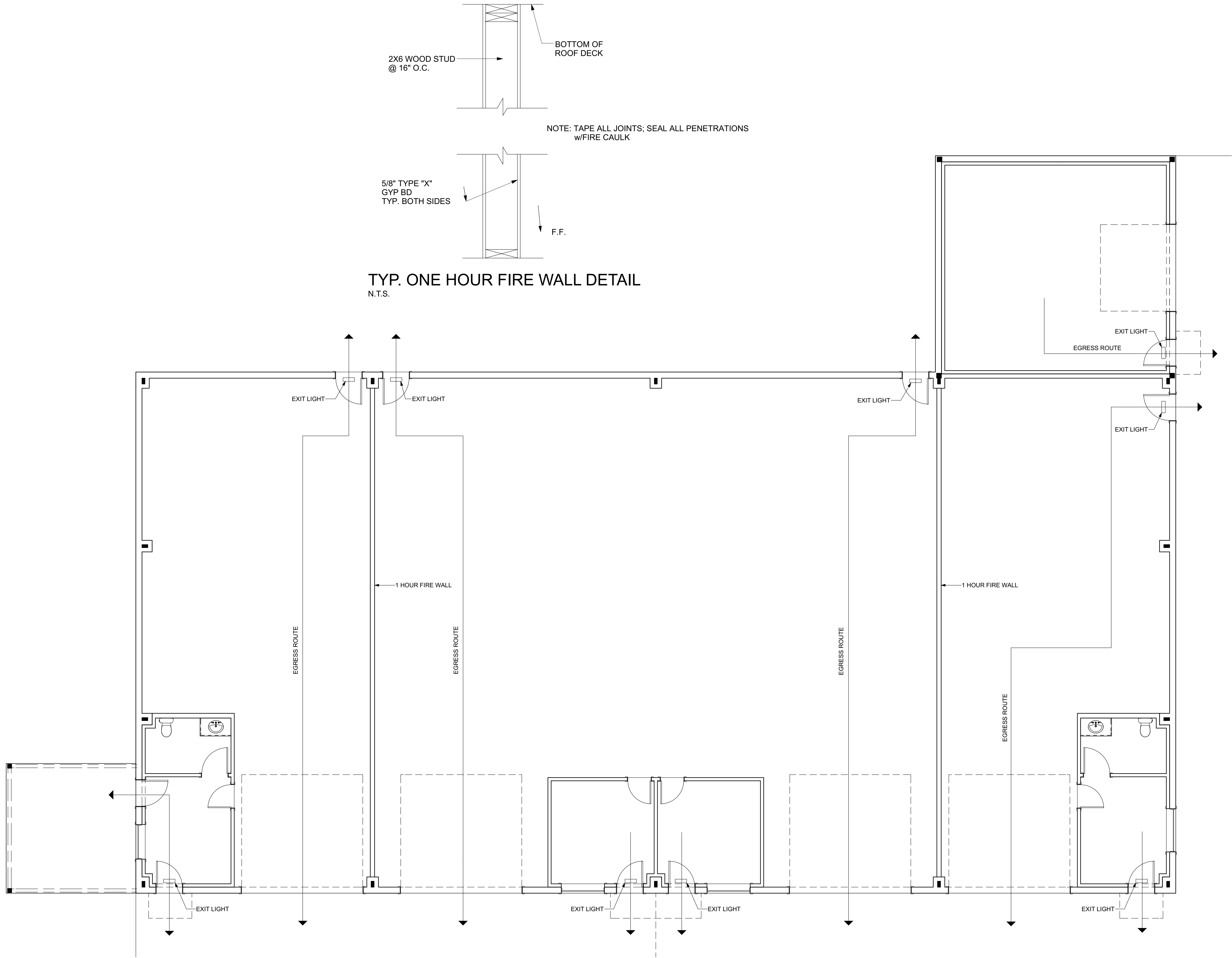
LIFE SAFETY PLAN SCALE:3/16" = 1'-0"
