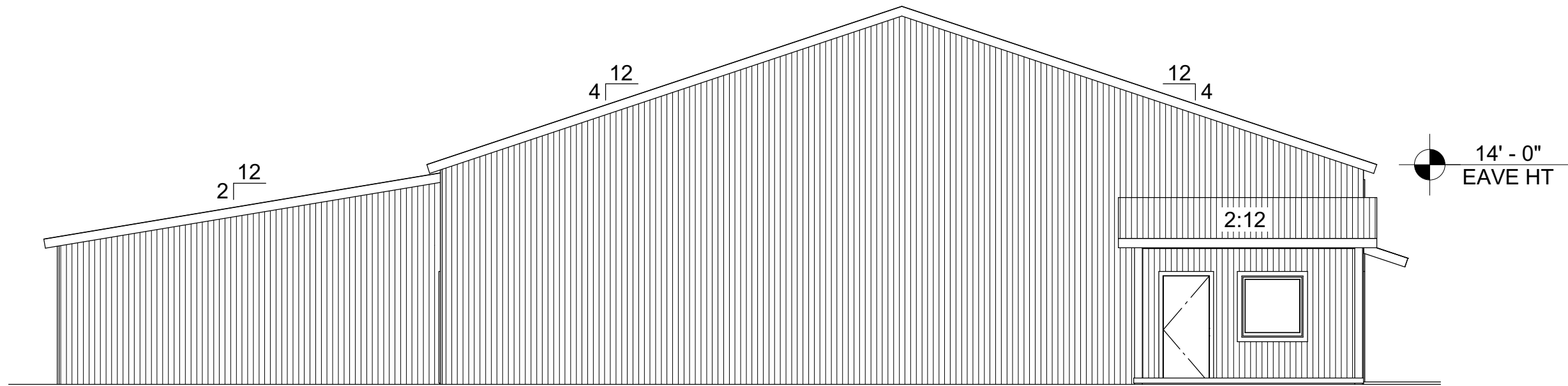
SOUTH ELEVATION SCALE:1/8"=1'-0"
