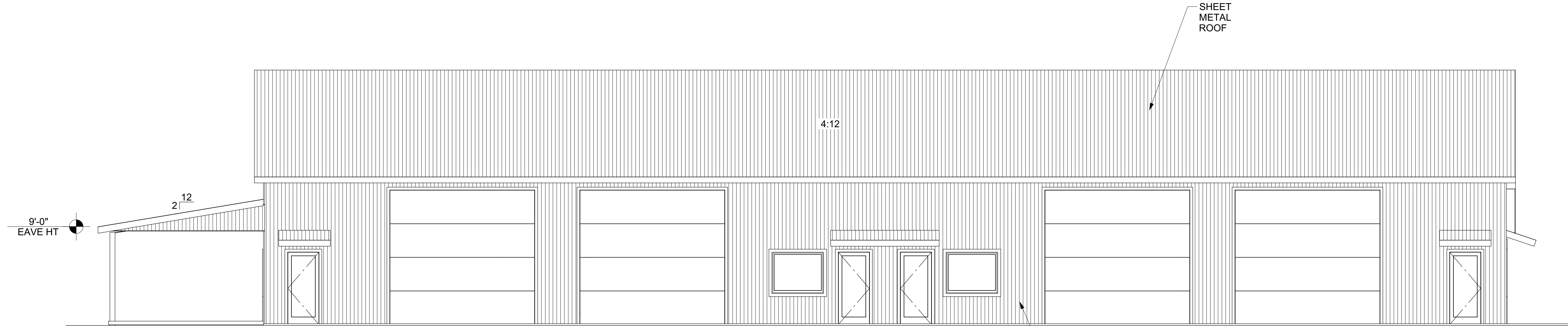
EAST ELEVATION SCALE:3/16"=1'-0"
