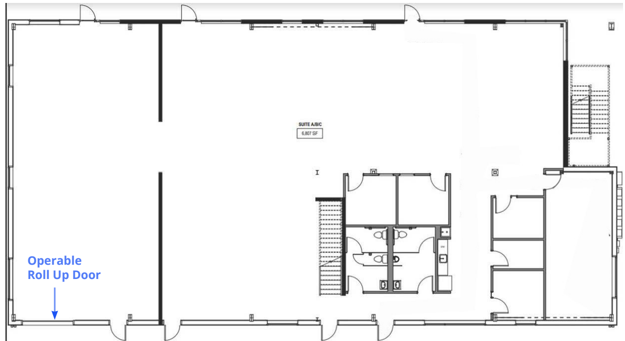
Second Floor
