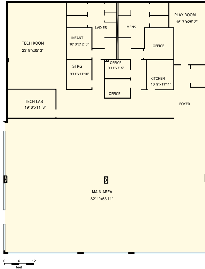
Main Floor Exterior Area 8599 sq. ft.
