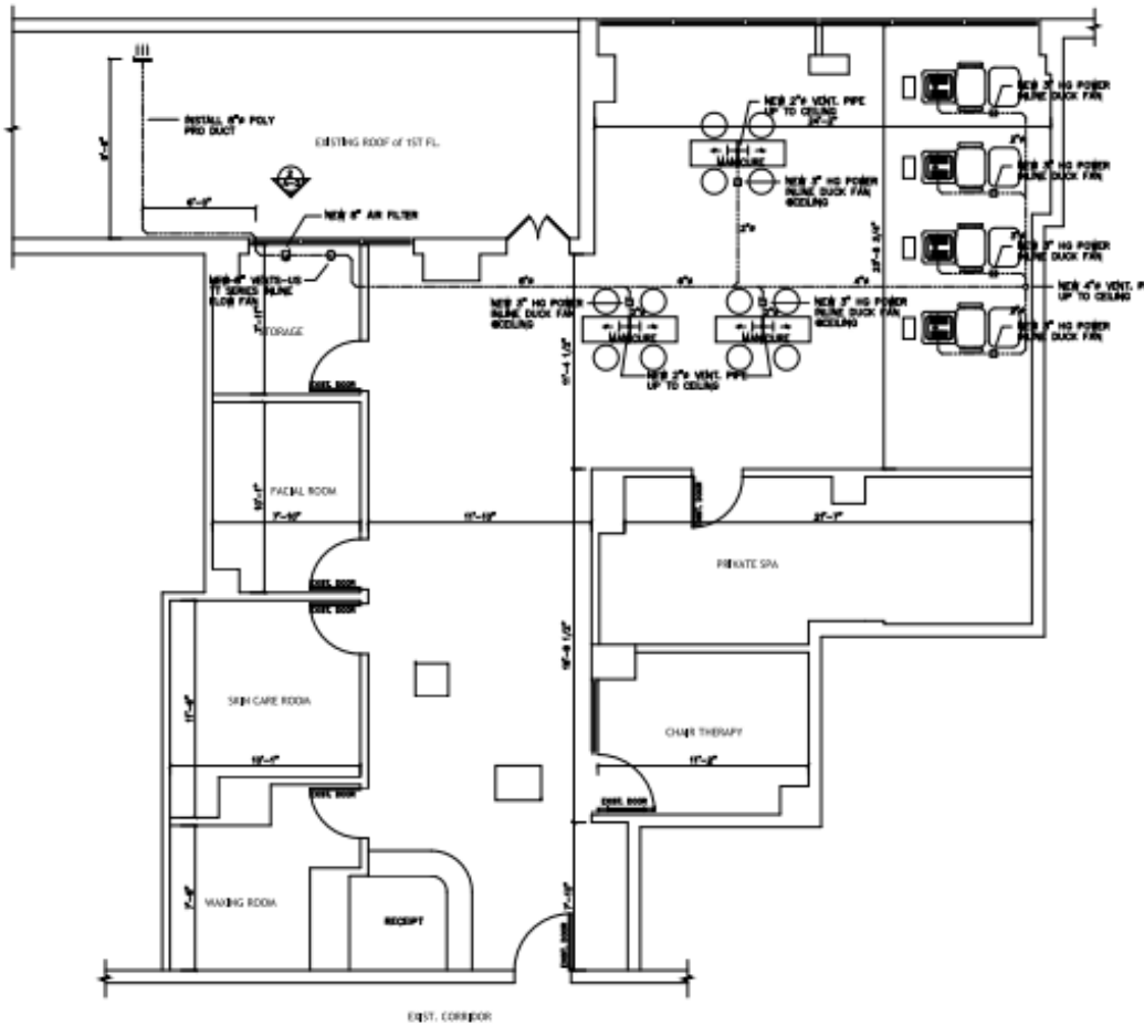
1 SECOND FLOOR PLAN SCALE 1/4" = 1'-0"
