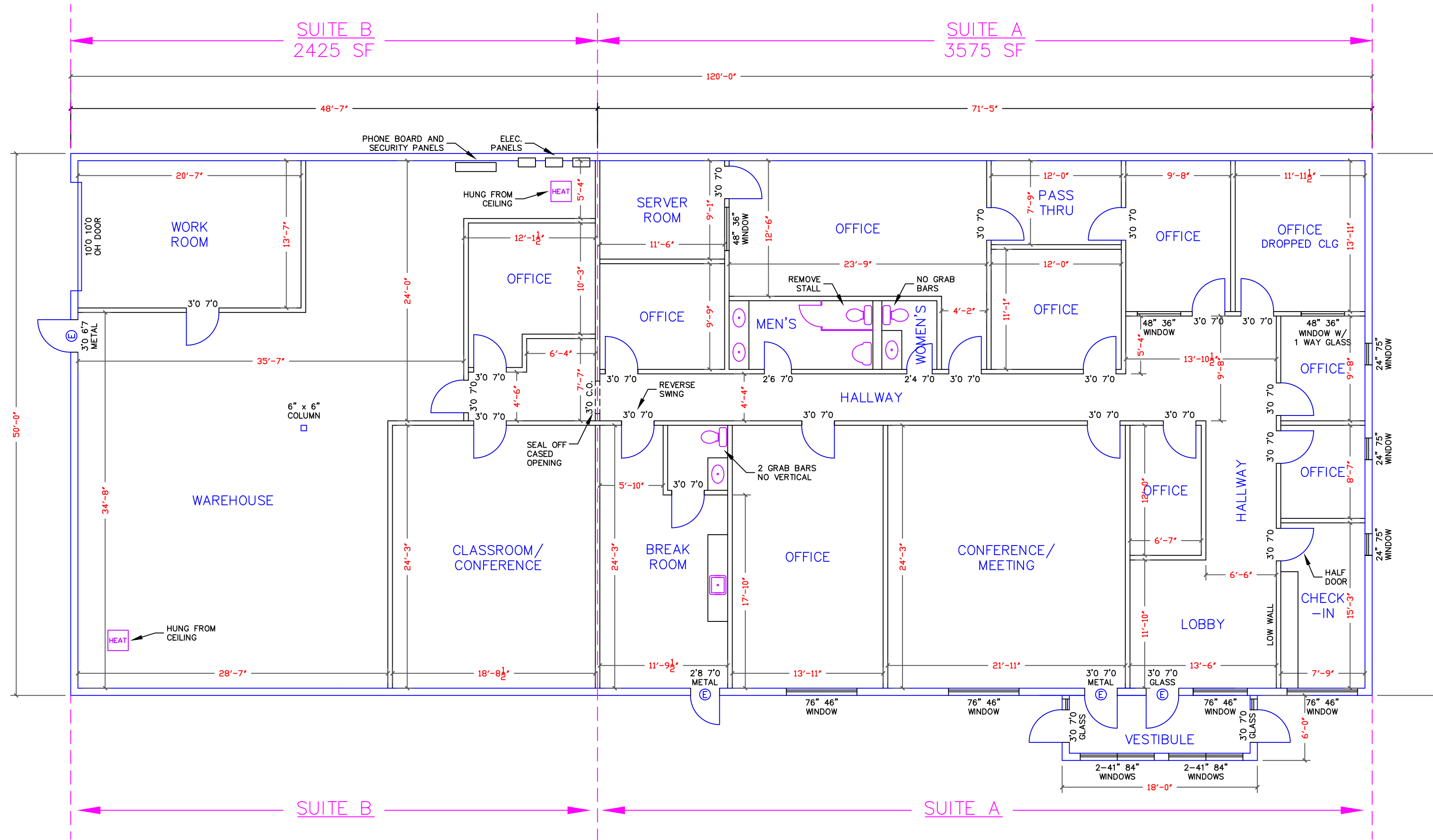
FLOOR PLAN 3575 SF OFFICE SPACE 3160 N. PORTLAND AVE., OKLAHOMA CITY, OK
