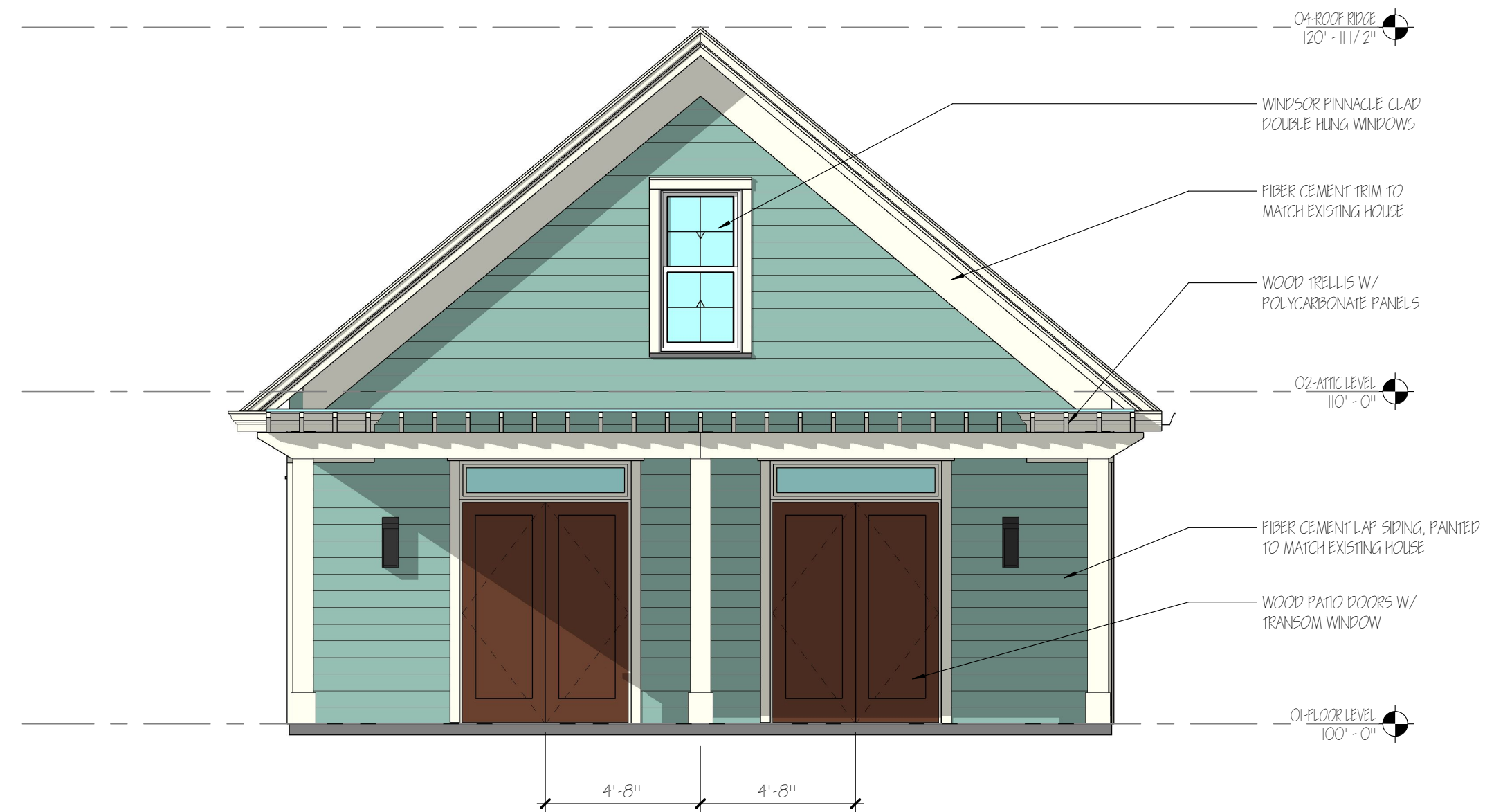
① ELEVATION - LOUNGE END 1/4" = 1'-0"
