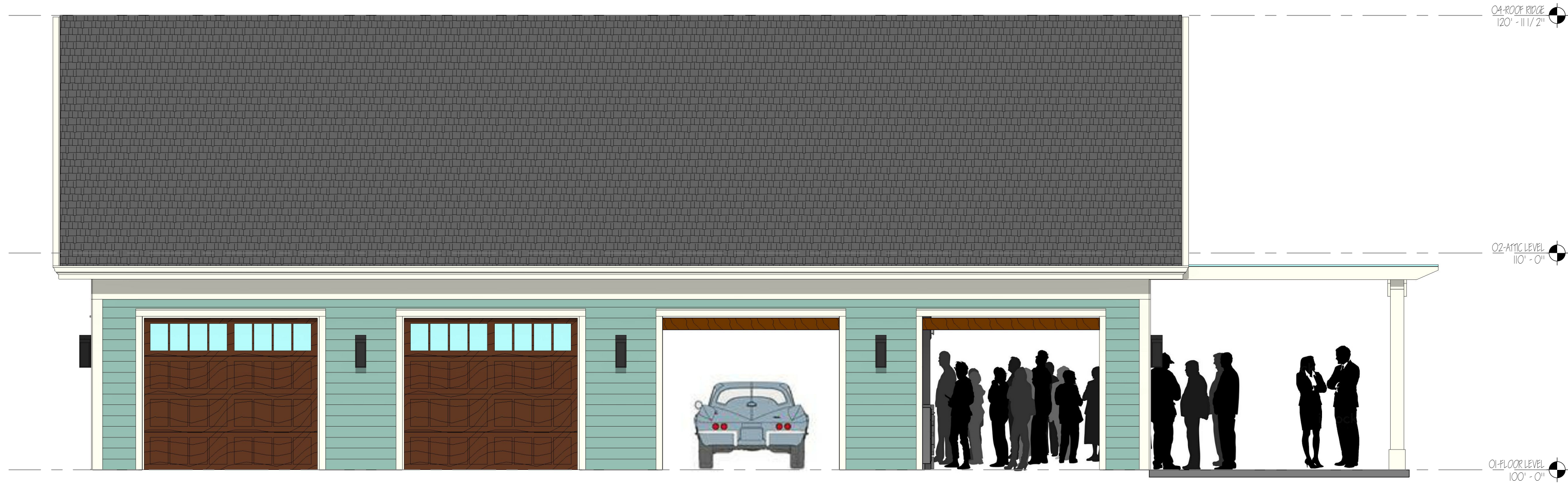
② FRONT ELEVATION - GARAGE DOORS OPEN 1/4" = 1'-0"
