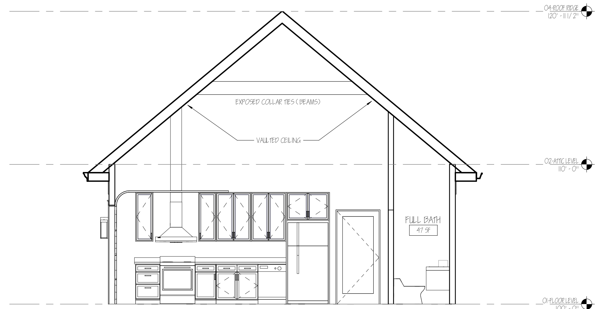
2 ELEVATION - KITCHEN CABINETS 1/4" = 1'-0"
