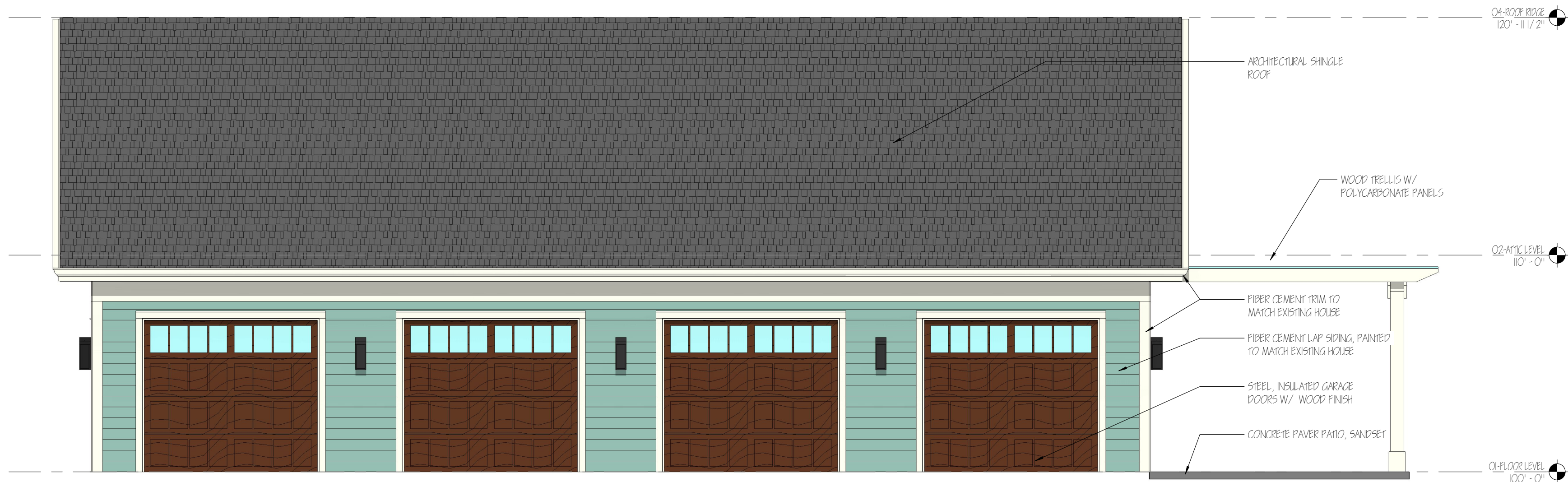
① FRONT ELEVATION - GARAGE DOORS CLOSED 1/4" = 1'-0"
