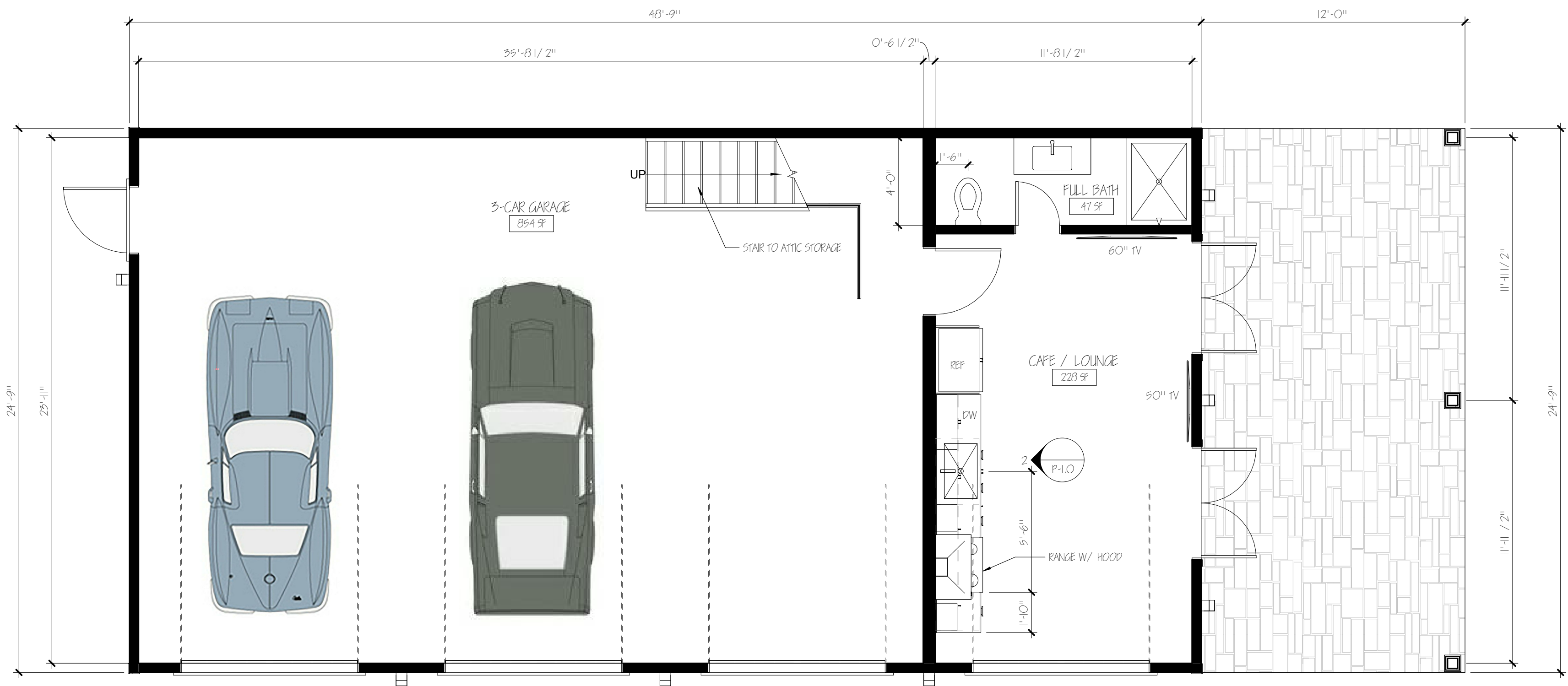
1 GARAGE PLAN 1/4" = 1'-0"
