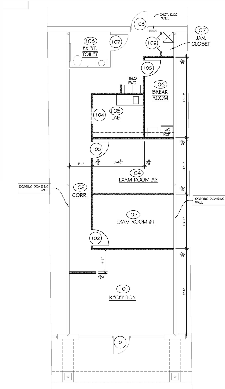
FLOOR PLAN 1/4" = 1'-0"
