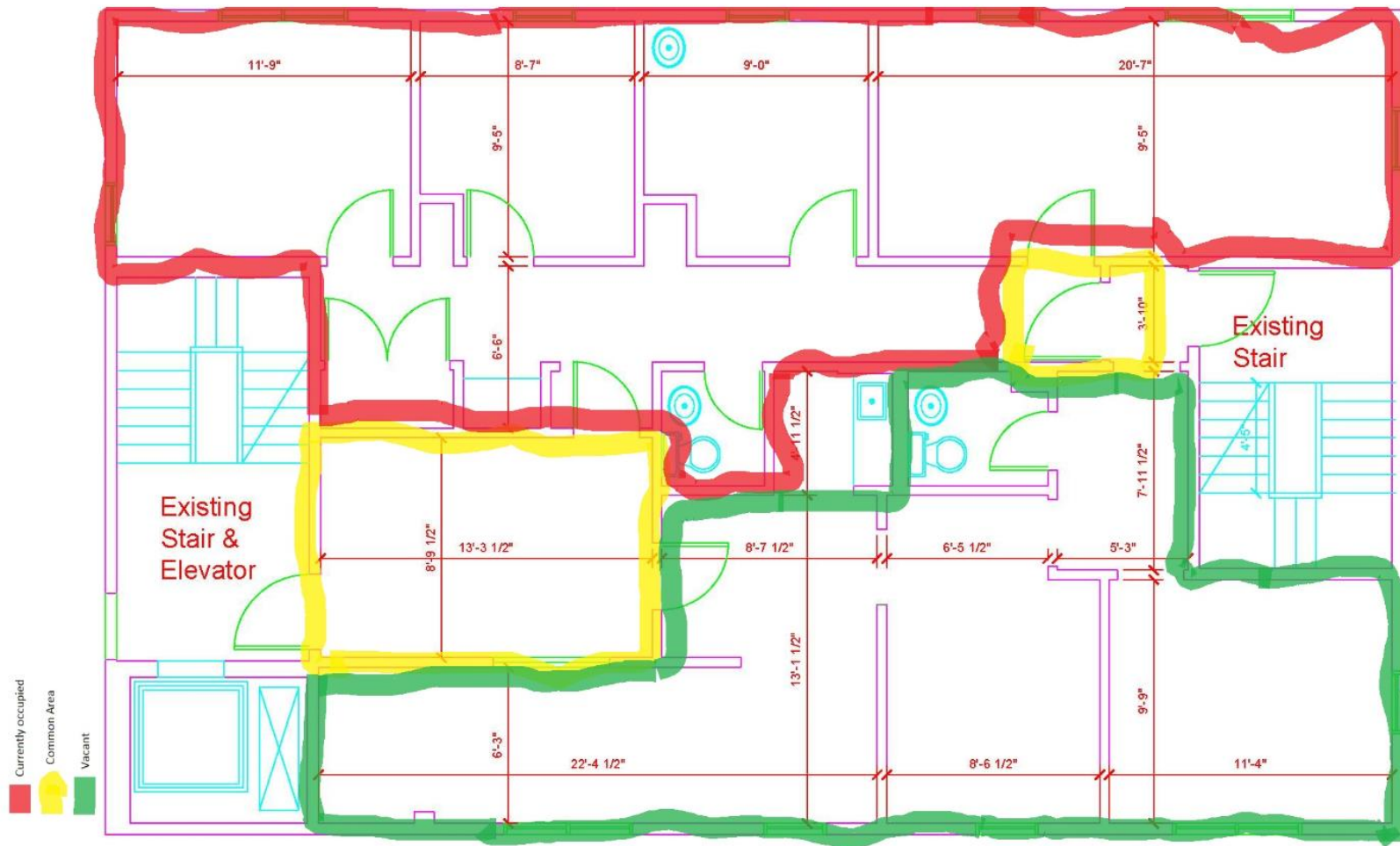
EXISTING SECOND FLOOR PLAN 22 LONG RIDGE ROAD
