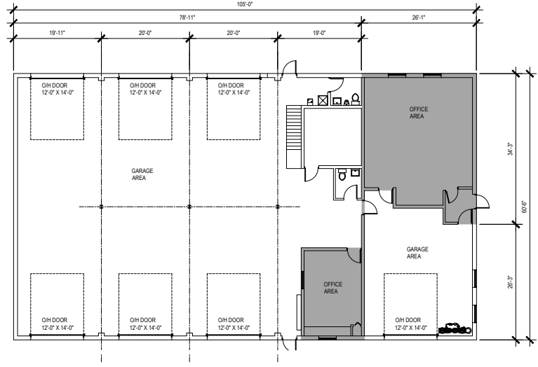
1 MAIN FLOOR PLAN 1/16" = 1'-0"
