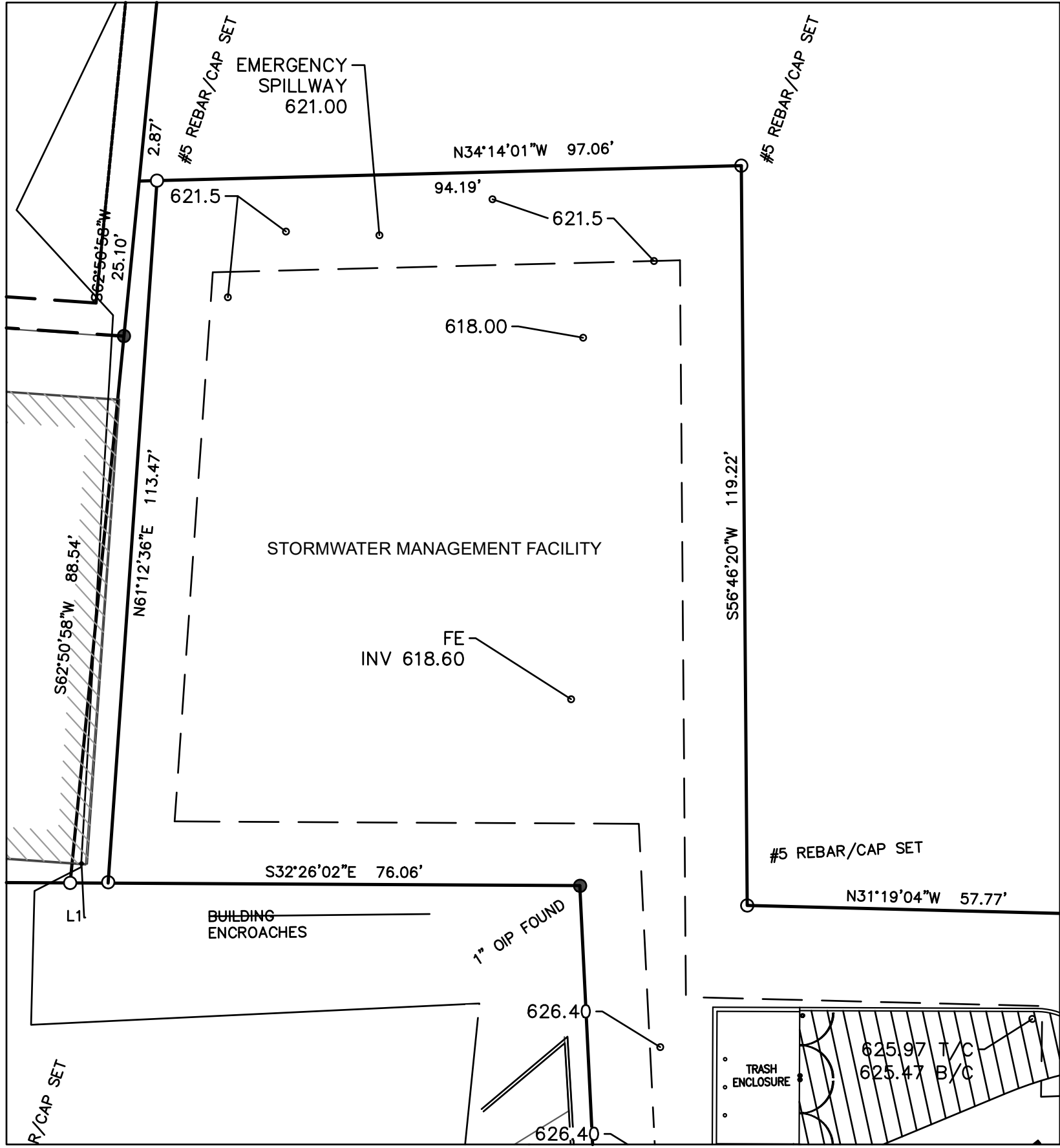
STORMWATER MANAGEMENT FACILITY
