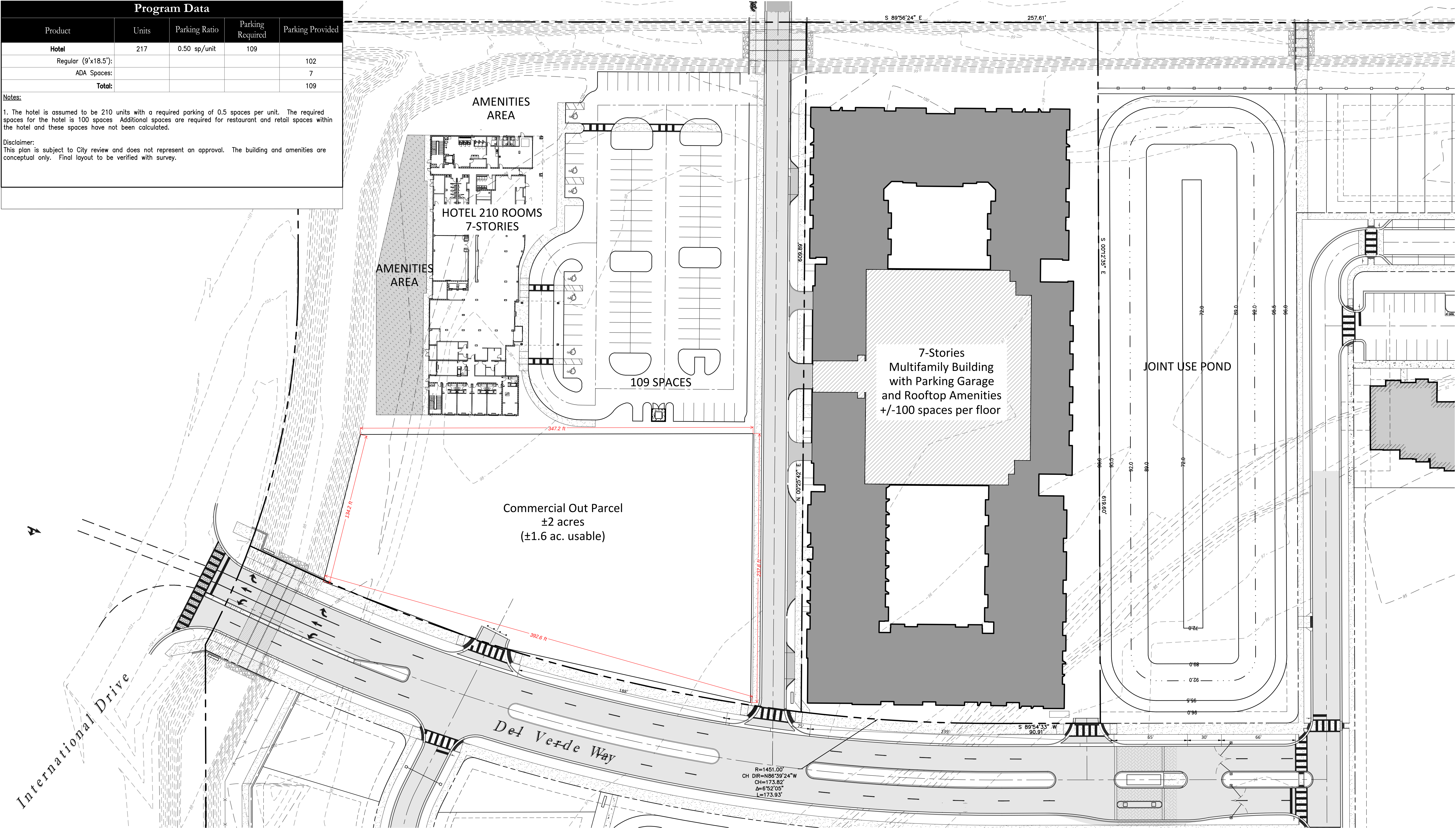
Conceptual Layout
