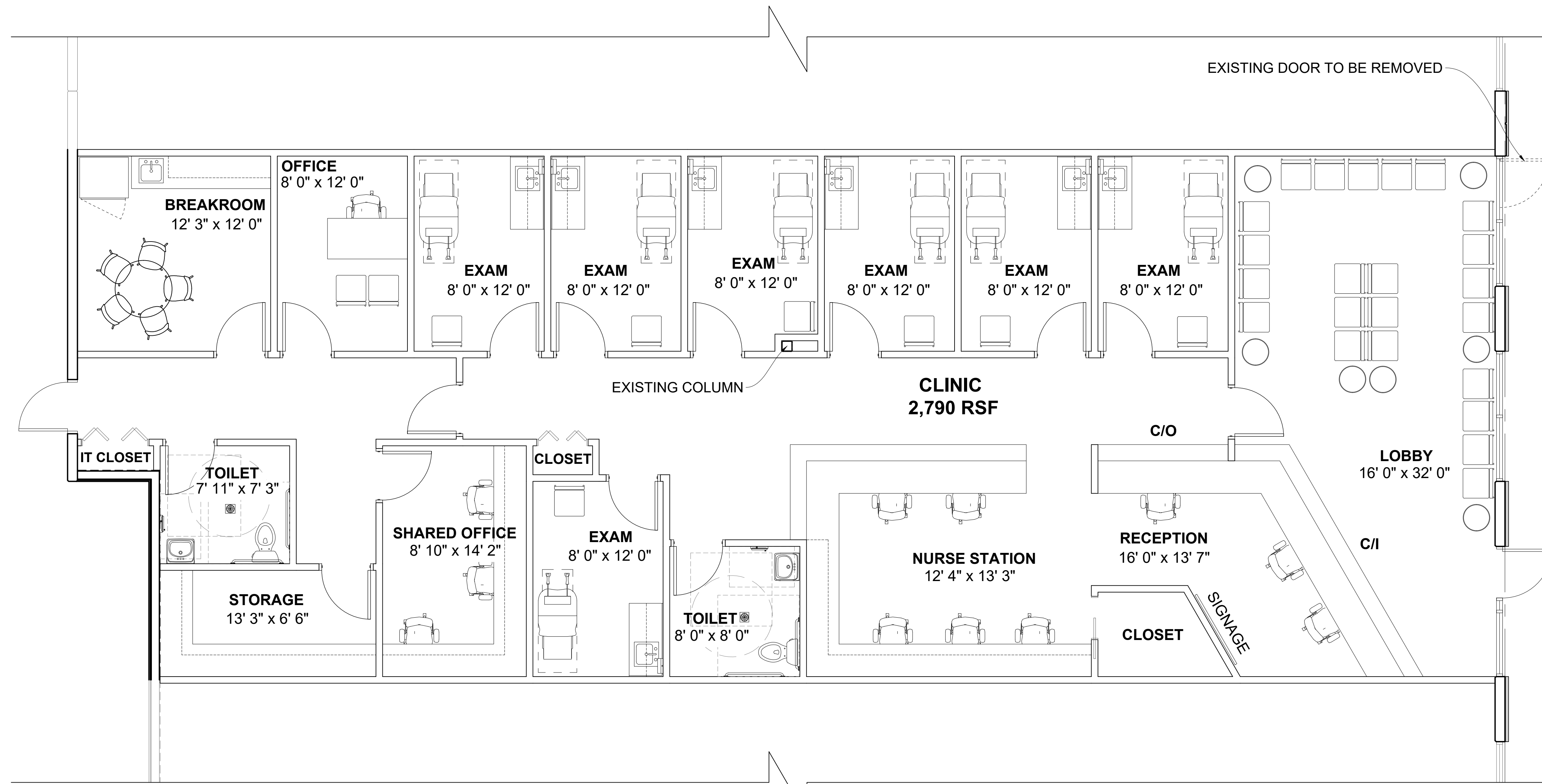
01 PRELIMINARY SPACE PLAN Scale: 1/4" = 1'-0"
