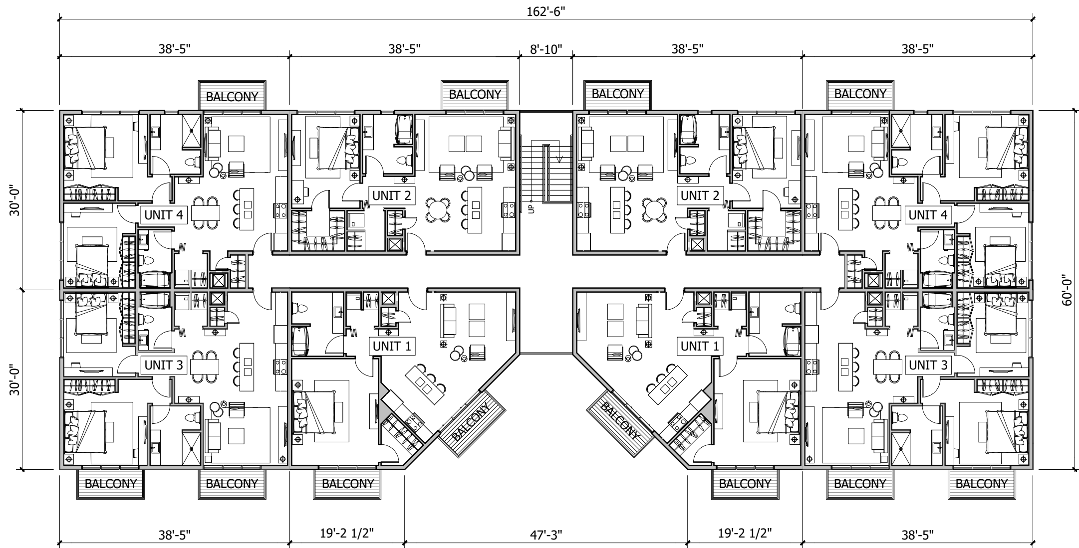
1 SECOND & THIRD FLOOR APARTMENT PLAN 1/16" = 1'-0"
