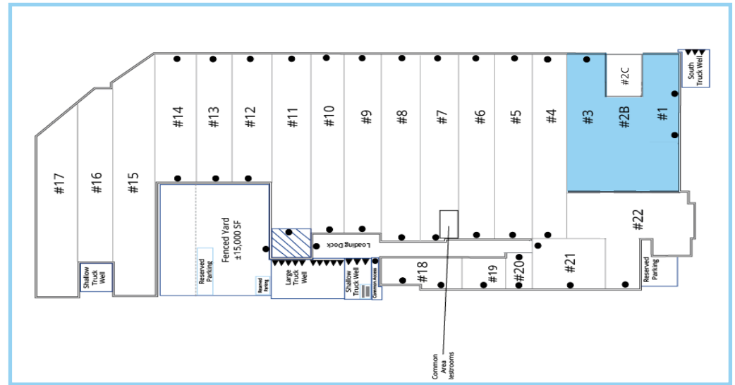
Proposed Siteplan
