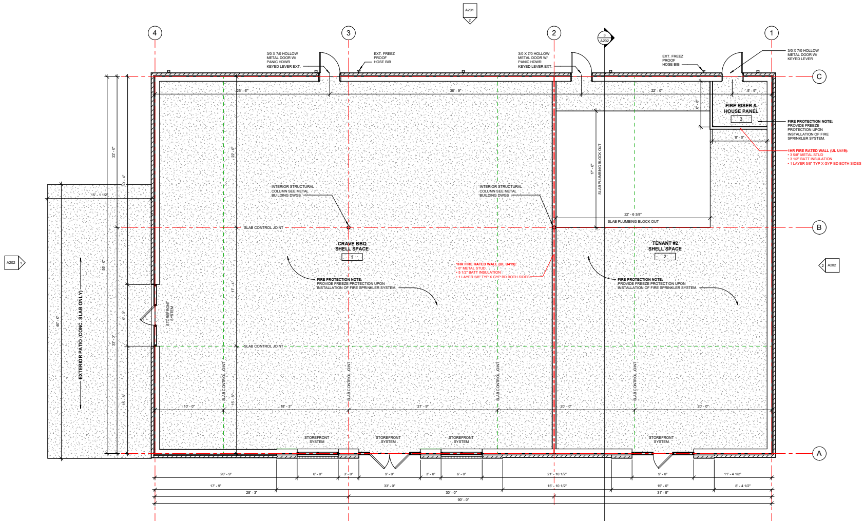
00 SHELL PLAN 1/4" = 1'-0"
