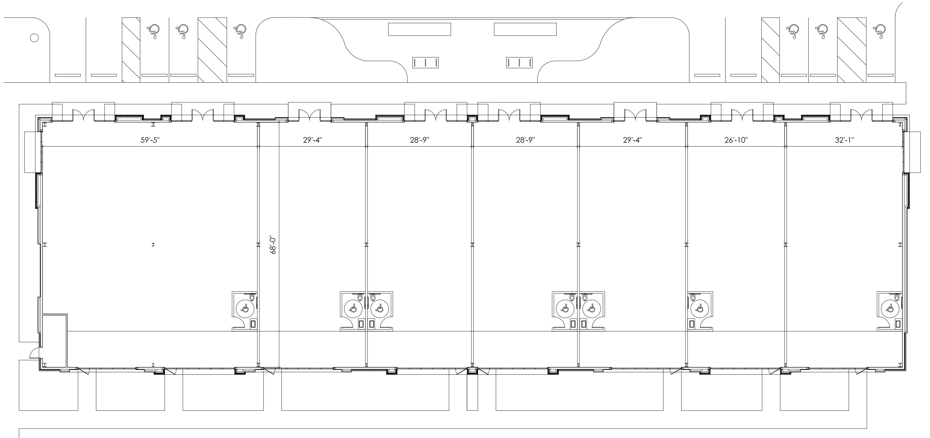
1 FLOOR PLAN SCALE: 1/16" = 1'-0"
