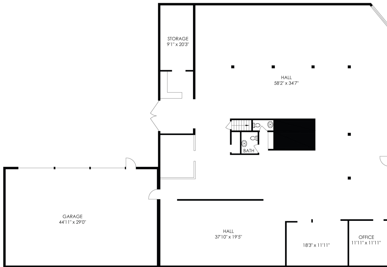
MAIN FLOOR
