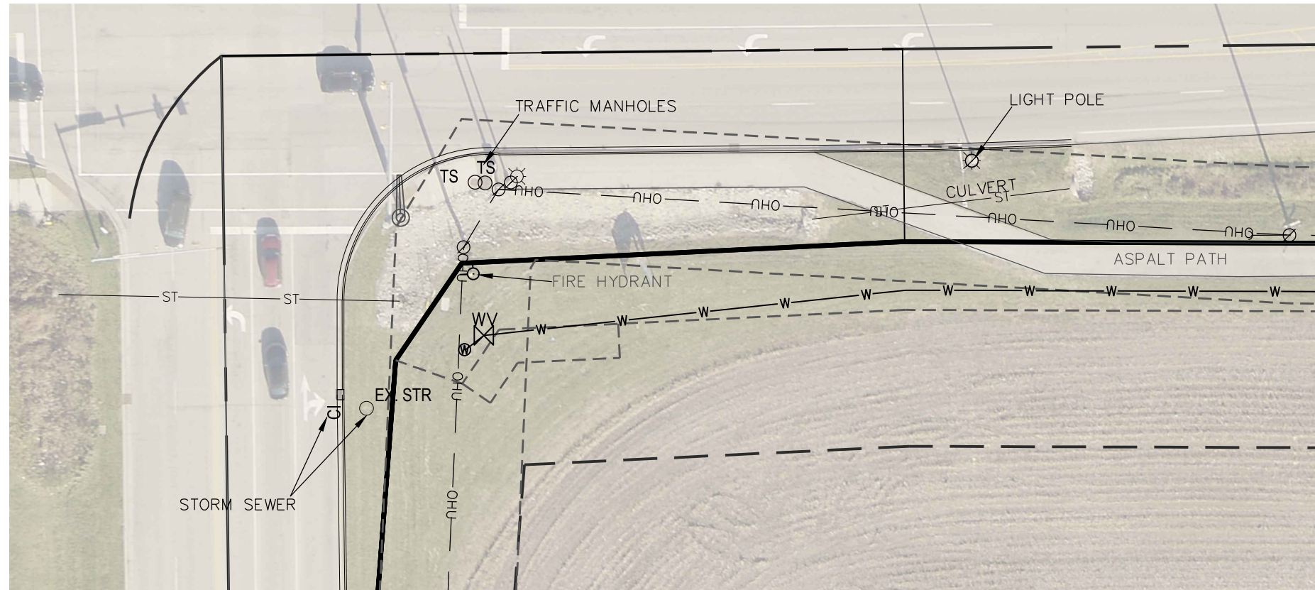
INTERSECTION DETAIL
