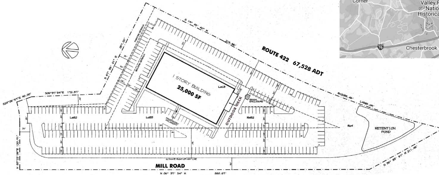
SITE PLAN SCALE: 1" = 40'
