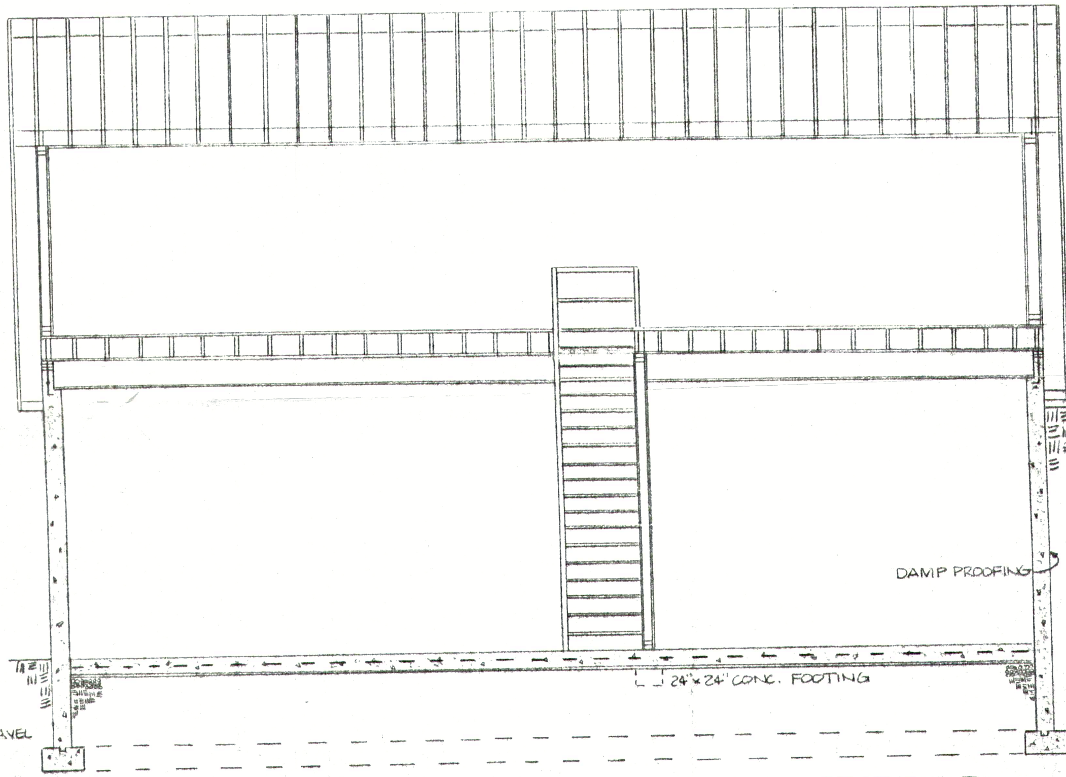
SECTION B
