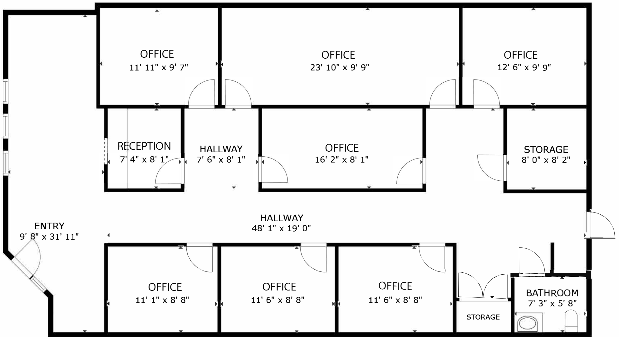
FLOOR PLAN
