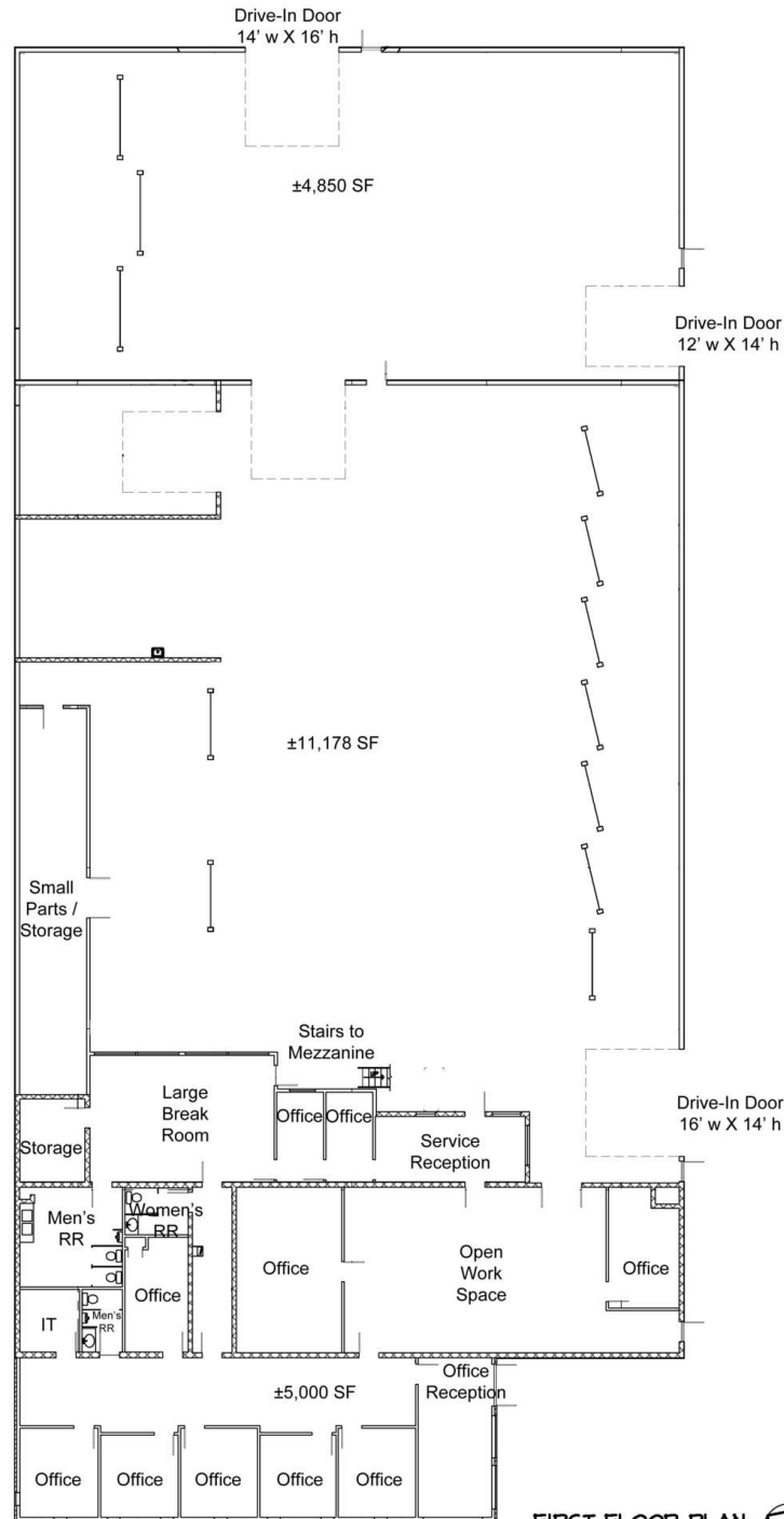
FIRST FLOOR PLAN 3/32" = 1'-0"
