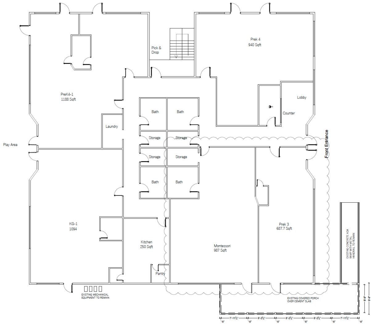
1 st Floor plan Was modified from 7 classrooms to 5 recently.
