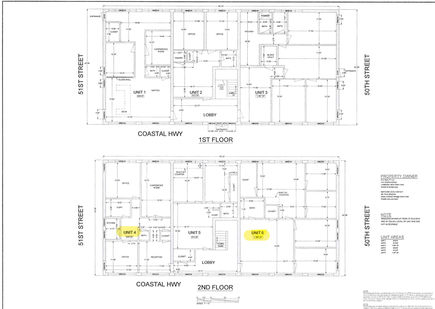
FLOOR PLAN
