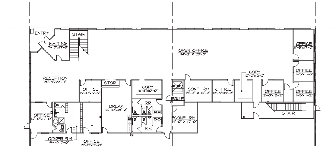
1ST FLOOR OFFICE PLAN
