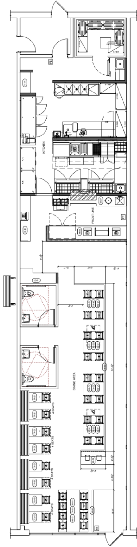
1 FURNITURE, FIXTURES & EQUIPMENT PLAN SCALE: 1/8" = 1'-0"
