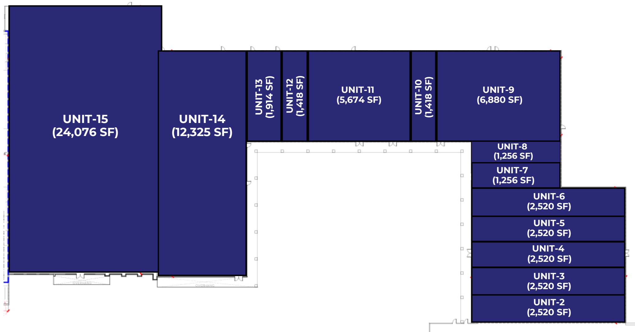
① BUILDING PLAN - RE-SIZED 1/16" = 1'-0"
