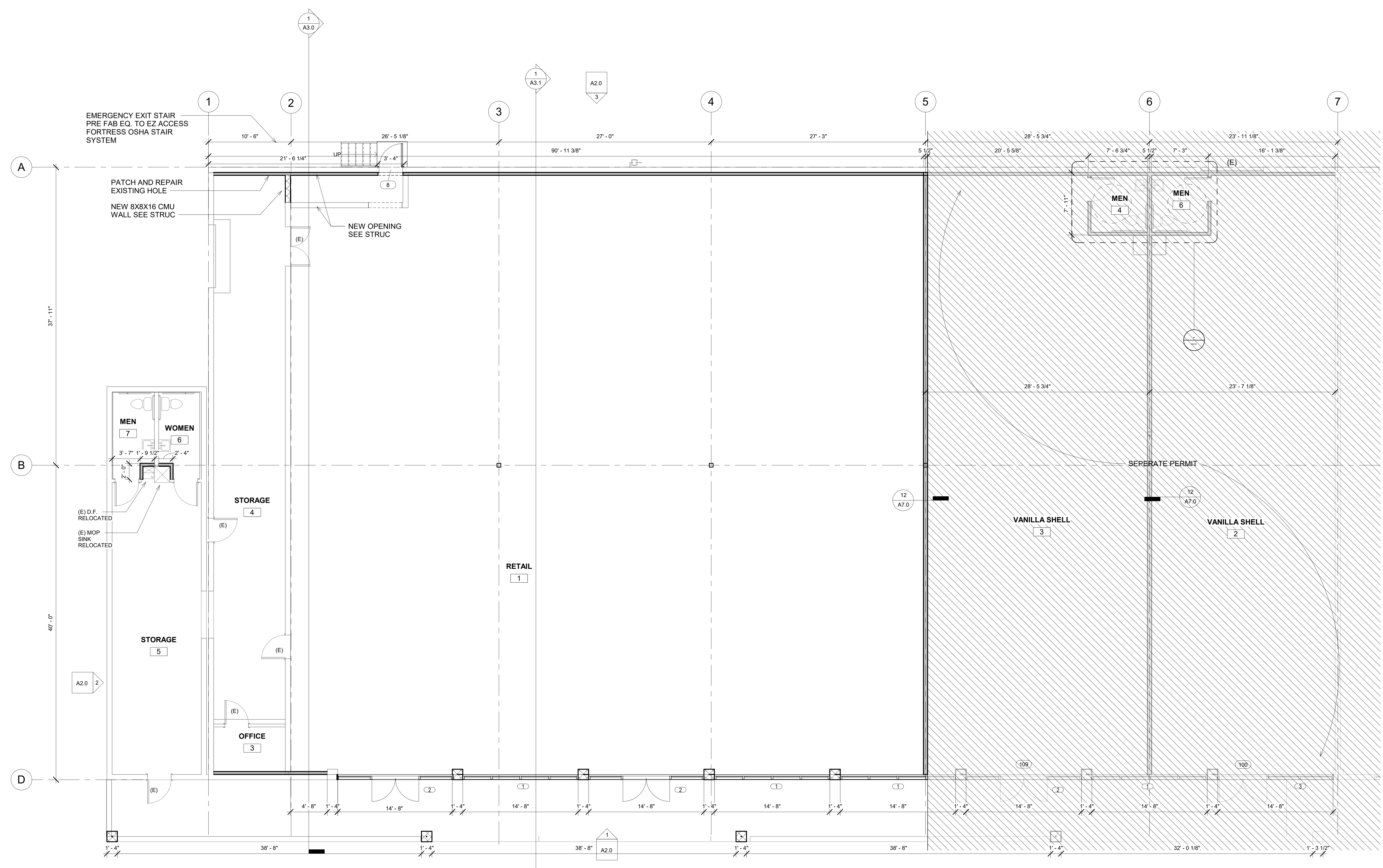
Dimension Floor Plan 3/16" = 1'-0"
