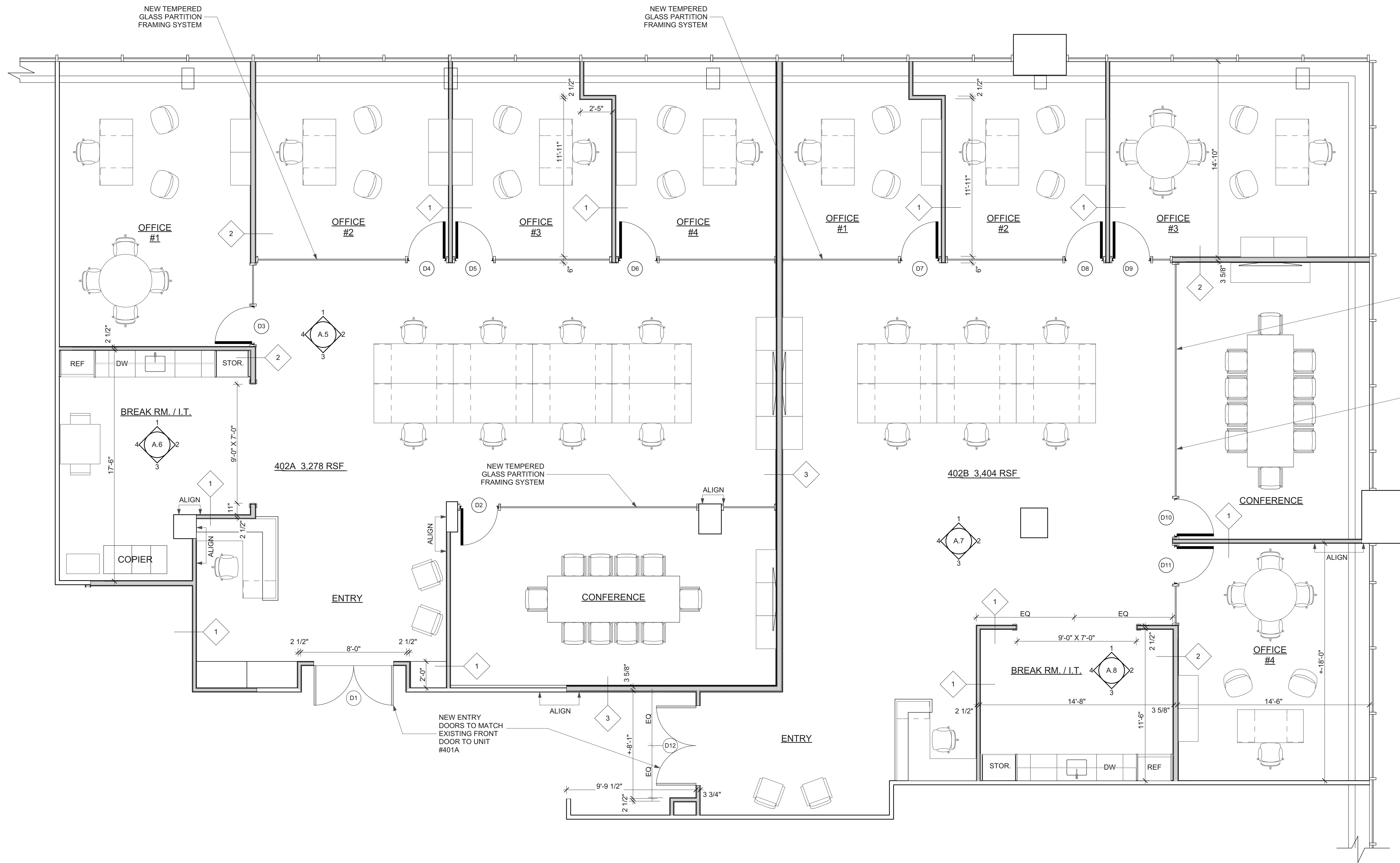
1 FOURTH FLOOR UNIT #402A & #402B SCALE: 1/4" = 1'-0"
