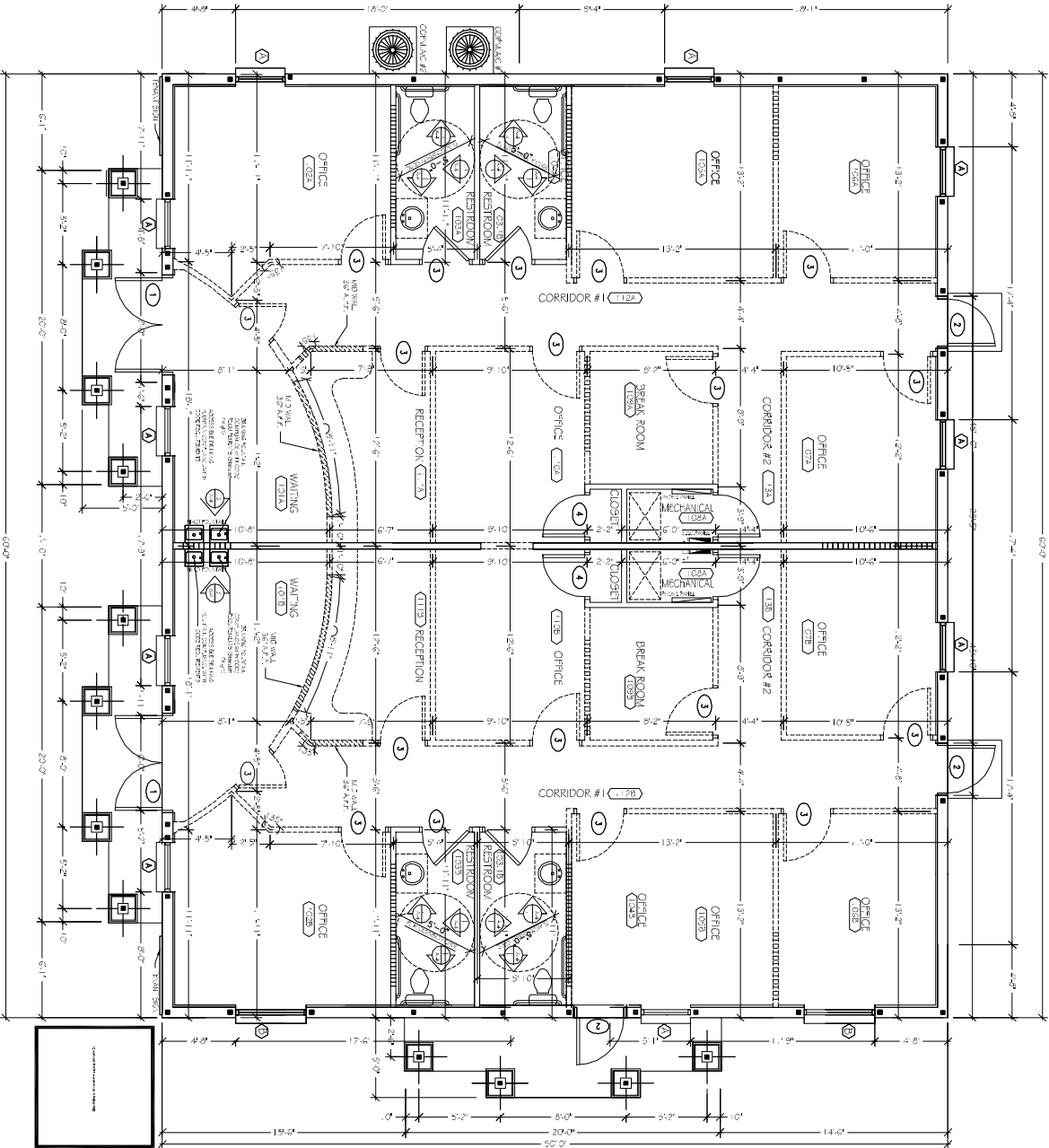
ORIGINAL FLOOR PLAN (2008) & NEW PROPOSED FLOOR PLAN SCALE: 1/8" = 1'-0"
