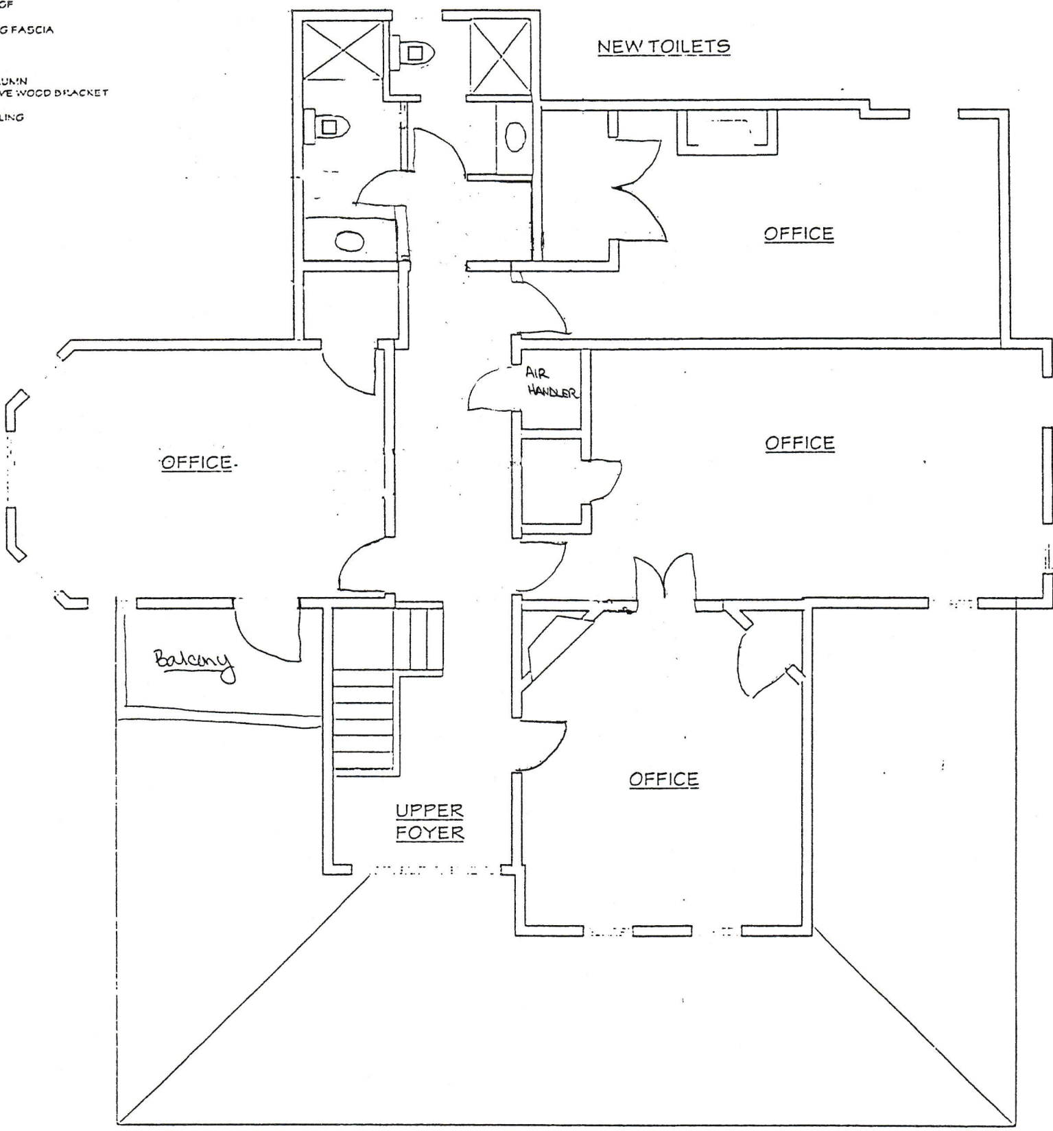
SECOND FLOOR PLAN 1/4"=1'-0"
